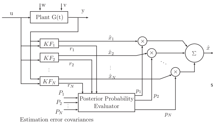
Figure 15: The MMAE architecture
