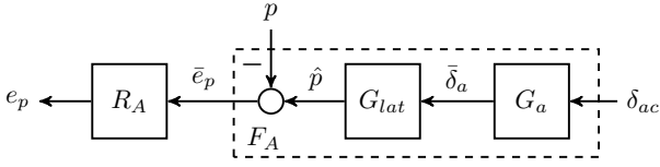
Figure 3: The architecture of Method A of the FDI algorithm.
