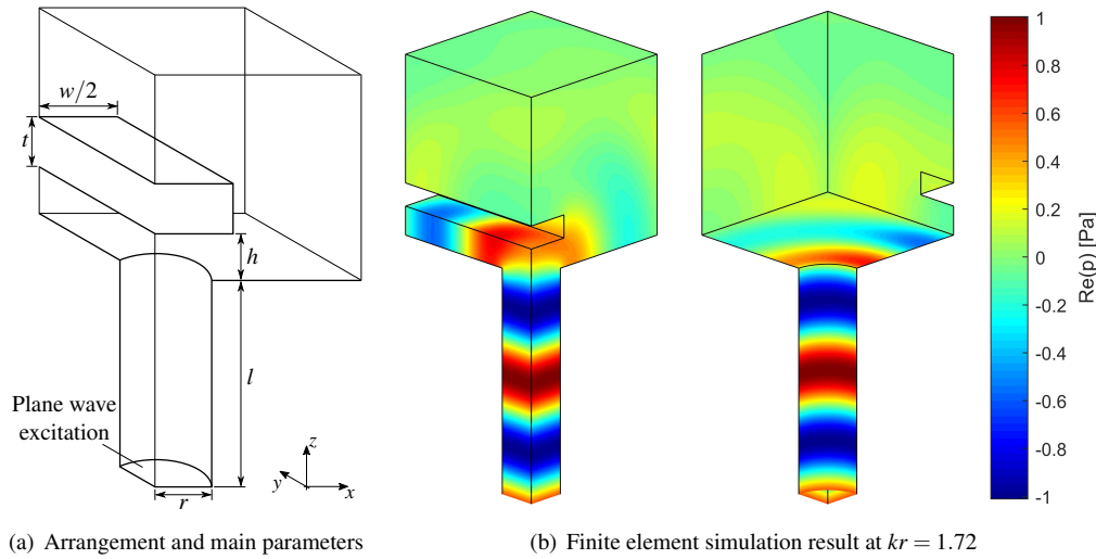
Figure 3. Finite element simulation of the effect of a sound bar partially covering a cylindrical tube
