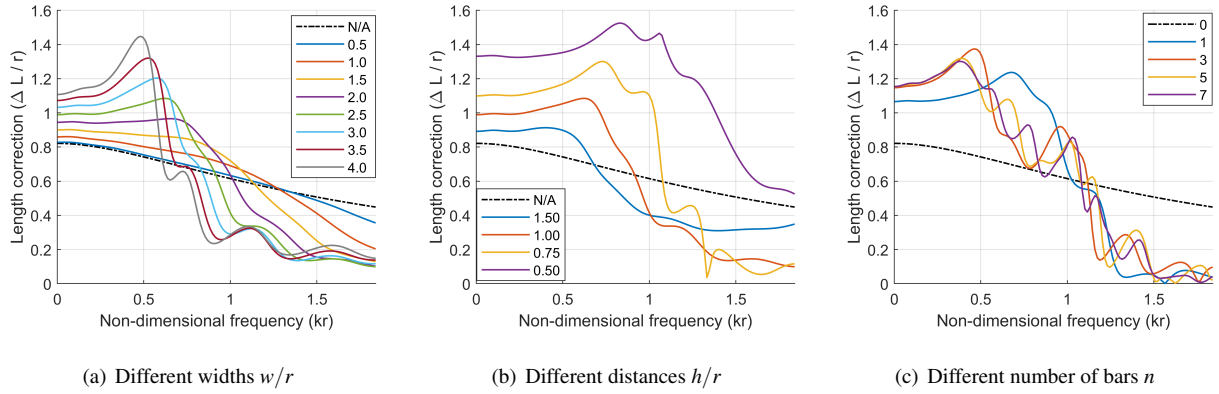
Figure 4. Length correction effect of sound bars partially covering the open end of a cylindrical tube in different geometrical arrangements. The dash-dotted line shows the reference setup without sound bars.
