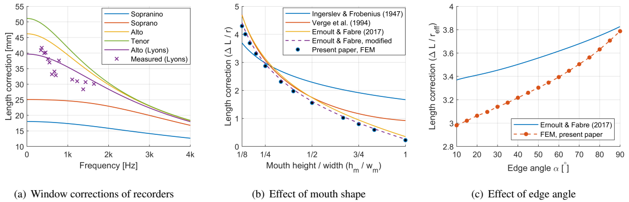
Figure 2. Simulation results of the length corrections of recorders and organ pipes compared to various models
