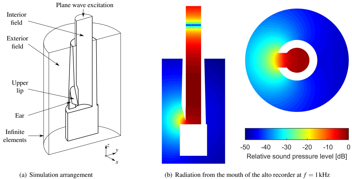
Figure 1. Finite element simulation of the sound radiation from the mouth of a recorder
