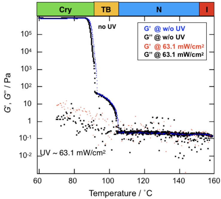
Figure S4: The variation of storage modulus ( G' ) and loss modulus ( G'' ) as a function of temperature measured in oscillatory mode on cooling either without UV illumination or under 63.1 \text{ mW/cm}^2 UV irradiance. The measuring conditions are: strain of 0.1%, angular frequency of 10 rad/s and temperature cooling rate of 1^{\circ}\text{C/min} . When UV illumination is made, both G' and G'' decrease dramatically in each phase.
