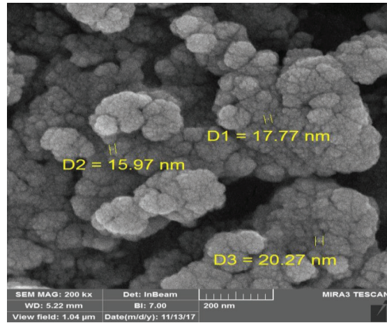
Fig. 3. SEM image of synthesized Fe_3O_4@Cumin
