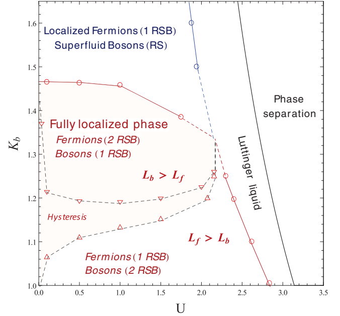
FIG. 12. (Color online) Phase diagram obtained by the Gaussian variational method in replica space, as a function of K_b and U = U_{\text{BF}}/\sqrt{v_b v_f} , for \tilde{D}_f = \tilde{D}_b = 0.005 and v_f/v_b = 1/3 . In the fully localized phase there is crossover between two regions where the order of replica symmetry breaking is reverted.
