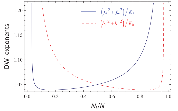
FIG. 2. (Color online) Density wave exponents for K_b = 1 and U_{\text{BF}}/v_0 = 1 , with v_0 = (v_f + v_b)/2 , as a function of the fraction of fermions. We take equal masses for both species, so that U_{\text{BF}}/v_0 is kept a constant for all fillings. Solid blue line, fermions. Red dashed line, bosons.
