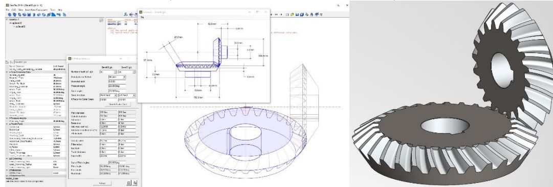
Figure 3 Designing of a helical bevel gear pair by GearTeq and Solidworks softwares ( m_{ax}=5 \text{ mm} , z_1=20 , z_2=30 , \alpha_0=20^\circ , \Sigma=90^\circ , right hand, \beta_0=20^\circ )
