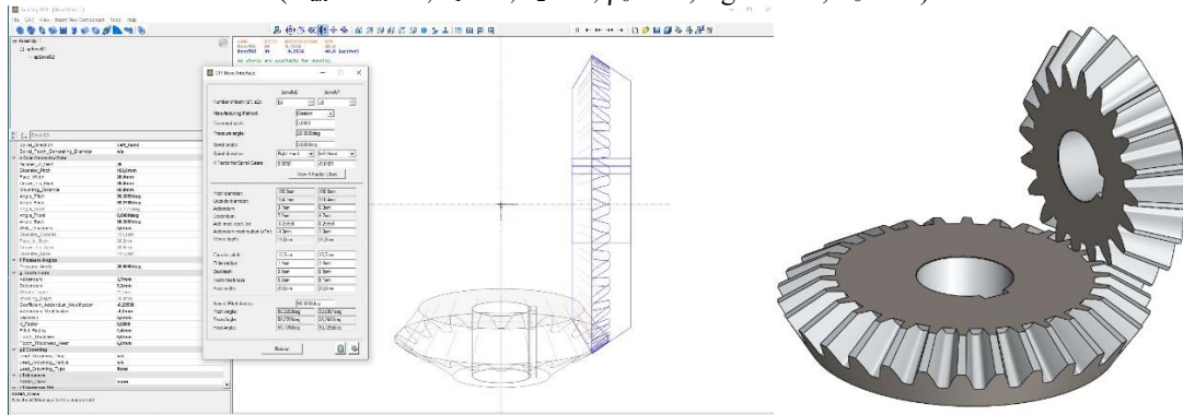
Figure 2 Designing of a bevel gear pair having straight tooth by GearTeq and Solidworks softwares ( m_{ax}=5 \text{ mm} , z_1=20 , z_2=30 , \alpha_0=20^\circ , \Sigma=90^\circ )
