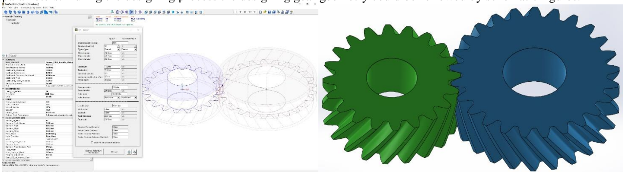
Figure 1 Designing of a helical gear pair by GearTeq and Solidworks softwares ( m_{ax}=15 \text{ mm} , z_1=20 , z_2=25 , \beta_0=30^\circ , right hand, \alpha_0=20^\circ )
