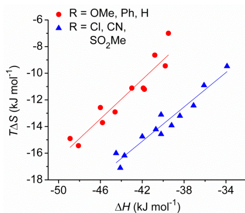
Figure 4. Correlation between the enthalpic and entropic contribution to the binding affinity of ligands ( S,S )-2–( S,S )-4 (R = OMe, Ph, H) and ( S,S )-5–( S,S )-7 (R = Cl, CN, SO 2 Me) toward the enantiomers of PEA and NEA in MeCN.
