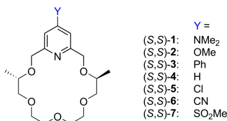
Figure 1. Enantiopure dimethyl-substituted pyridino-18-crown-6 ethers with various substituents at position 4 of the pyridine ring.
