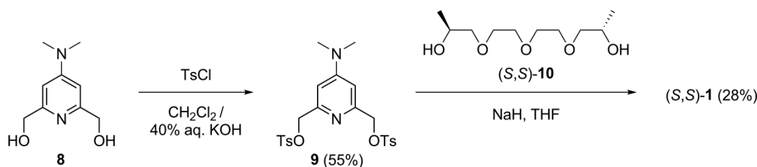
Scheme 1. Synthesis of crown ether ( S,S )-1.
