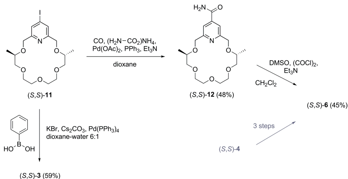
Scheme 2. Synthesis of crown ether (S,S) -3 and an alternative synthetic route for the preparation of macrocycle (S,S) -6 (the reported procedure [32] starts from crown ether (S,S) -4).
