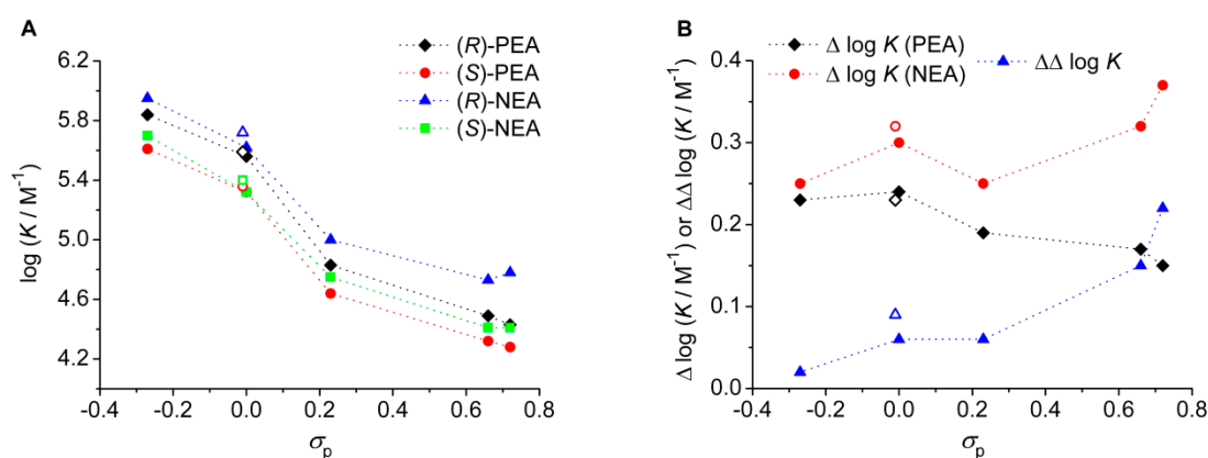
Figure 3. \log K values (A) and \Delta \log K values and their difference ( \Delta \Delta \log K = \Delta \log K (NEA) – \Delta \log K (PEA)) (B) as a function of the Hammett parameter for ligands ( S,S )-2–( S,S )-7 and PEA and NEA in MeCN. The corresponding values for ligand ( S,S )-3 are indicated with hollow symbols. The dashed lines are shown as a guide for the eye.
