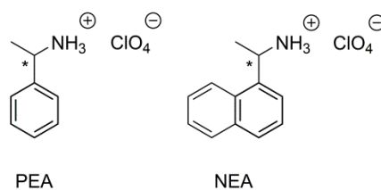
Figure 2. Chiral ammonium salts used as guests for enantiomeric recognition studies.
