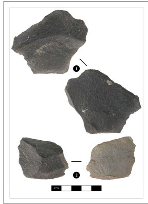
Fig. 10.: Selected artefacts. 1=Unretouched knife or side-scrapers.
