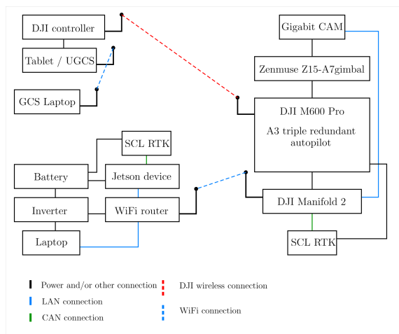
Figure 1: Hardware concept of the Forerunner UAV system
