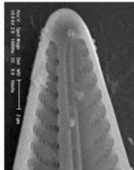
Figs 9–12. Navicula hasta Pantocsek. 9–12 = SEM, internal view of the valve.
