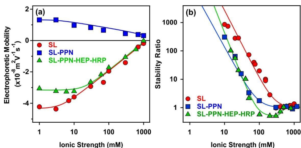
Fig. 4 (a) Electrophoretic mobility and (b) stability ratio of SL, SL-PPN, SL-PPN-HEP-HRP particles as a function of the ionic strength adjusted with NaCl. The measurements were carried out at pH 4 and the particle concentration was 10 mg/L.
