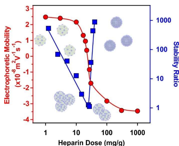
Fig. 1. Electrophoretic mobility (red circles) and stability ratio (blue squares) data of the SL-PPN particles as a function of the HEP dose. The measurements were carried out at pH 4 and 1 mM ionic strength adjusted by NaCl. The mg/g unit refers to mg of HEP per 1 g of the particles. The solid lines serve to guide the eyes.
