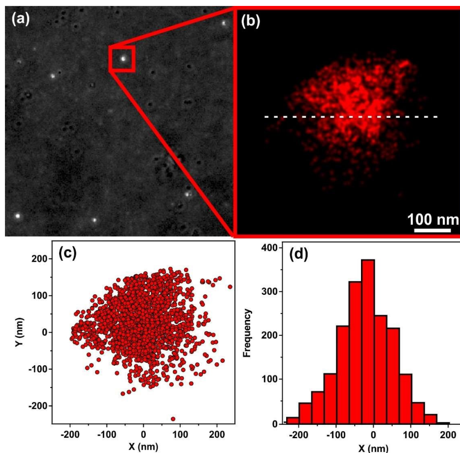
Fig. 2 Transmitted light image of the particles on glass surface (a) and dSTORM picture of the marked focal point (b). Blinking events of the fluorophores were plotted along the X and Y axes (c) and the frequency of blinking events was plotted as a function of the distance (d) from the white dashed line shown in the Fig 2b.
