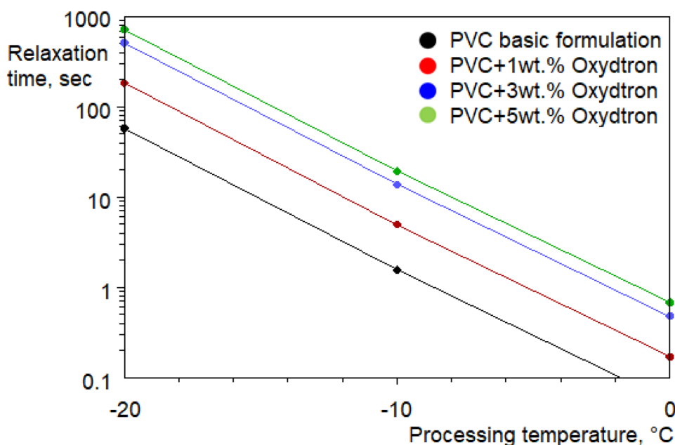
Fig. 10 The relaxation time for plasticized poly(vinyl chloride) containing Oxydtron as a function of temperature
