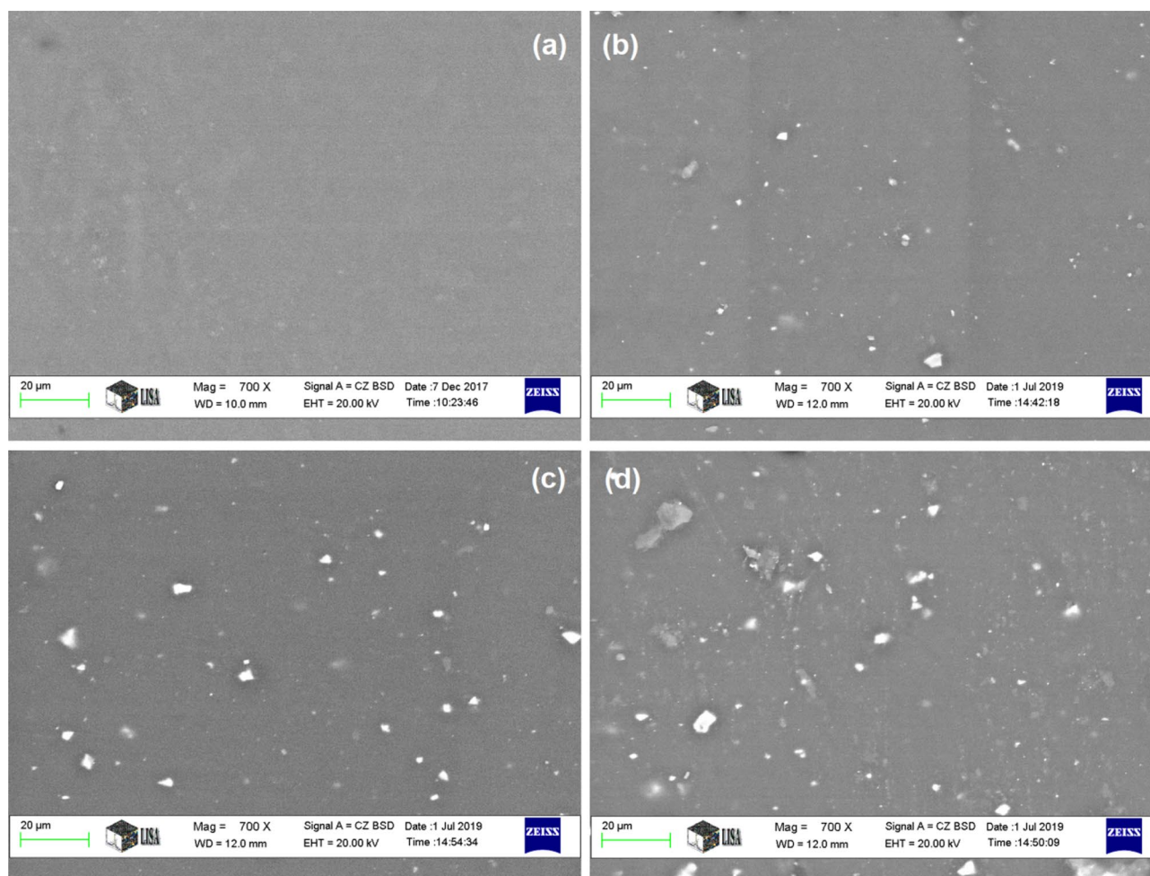
Fig. 2 SEM analysis images for dispersion of Oxydron in the poly(vinyl chloride), where (a) Poly(vinyl chloride) basic formulation, (b), (c), and (d) Poly(vinyl chloride) containing 1wt.%, 3wt.%, and 5wt.%, Oxydron respectively
