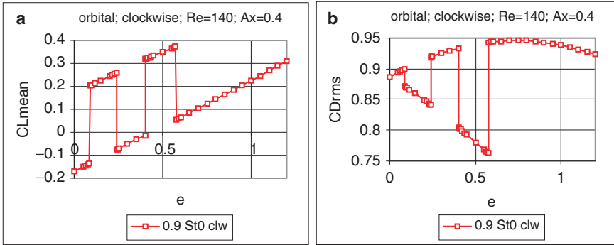
Fig. 2 Time-mean value of lift (a) and rms value of drag (b) versus ellipticity
