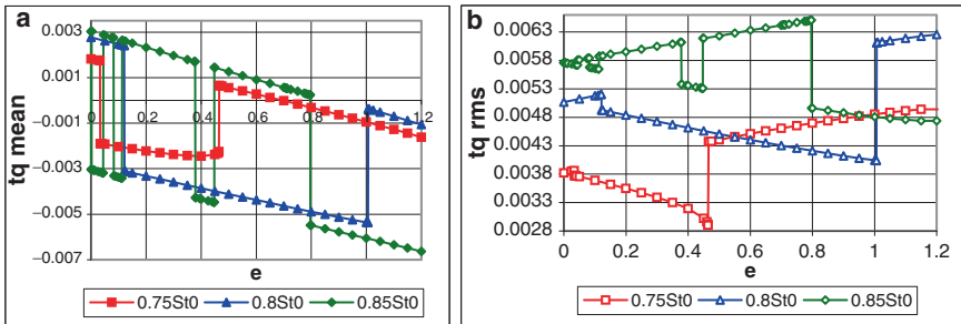
Fig. 3 Time-mean and rms values of torque coefficient versus e ( Re = 160 ; A_x = 0.4 )
