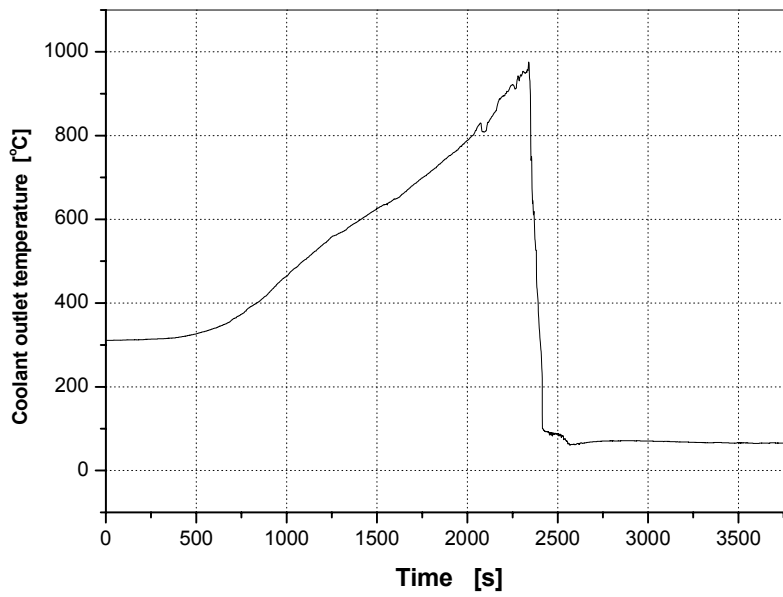
Fig. 41 TCOUT: coolant outlet temperature
