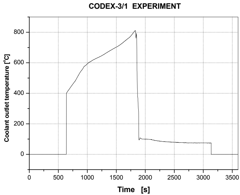
Fig. 20 TCOU: coolant outlet temperature
