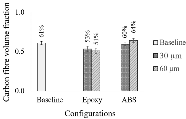
Fig. 11. Carbon fibre volume fraction ( V_{fc} ) in the baseline and film interleaved hybrid laminates. (For interpretation of the references to colour in this figure legend, the reader is referred to the web version of this article.)
