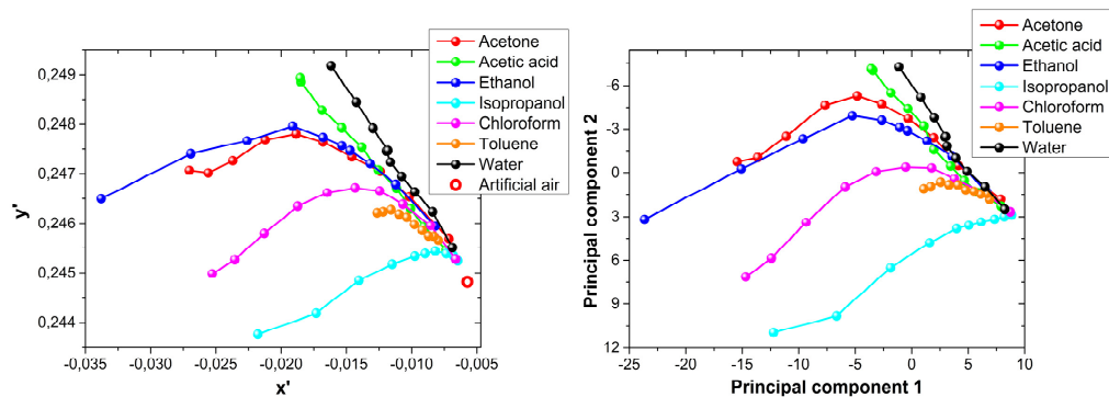
Fig. 6. (a) 2D transformed version of the 3D chromaticity diagram containing the results of the vapor sensing experiment. The red circle shows chromaticity point of the initial wing reflectance in artificial air from which the different vapor concentrations can be found right to left in ascending order. (b) The results of the PCA using the same vapor sensing data set.
