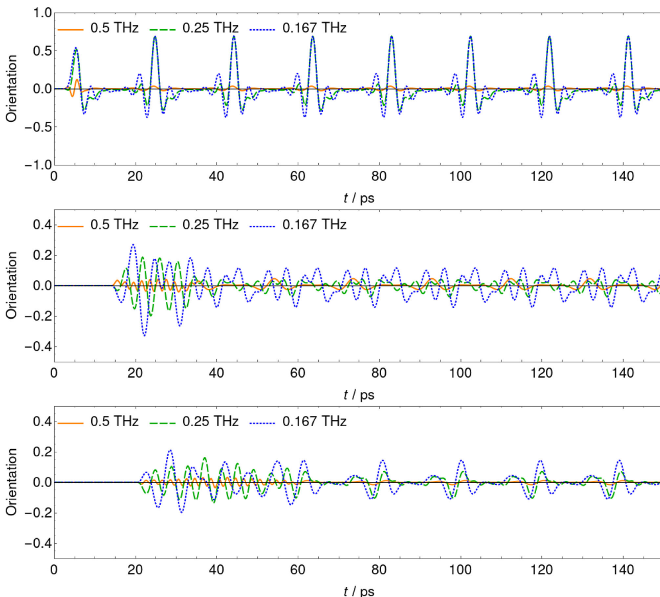
FIGURE 10 Effect of THz pulse parameters on the orientation of \text{CH}_3\text{F} . The frequency ( \nu ), intensity ( I ), and FWHM was varied, keeping the total pulse energy, I \times \text{FWHM} constant. T/K = 5 and \text{CEP} = \pi/2 were used for all panels. The other pulse parameters of the top panel: \text{FWHM} = 2 ps, I = 5 \times 10^{-4} \text{TW cm}^{-2} , pulse position was 5 ps; middle panel: \text{FWHM} = 10 ps, I = 1 \times 10^{-4} \text{TW cm}^{-2} , pulse position was 25 ps; bottom panel: \text{FWHM} = 20 ps, I = 5 \times 10^{-5} \text{TW cm}^{-2} , pulse position was 40 ps
