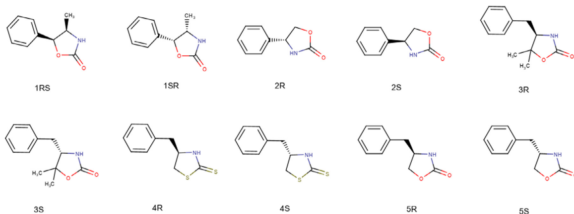
Fig. 1. The chemical structure of the analytes.
