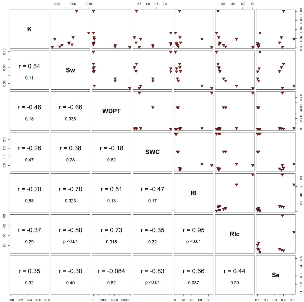
Fig. 10. Scatterplot Pearson-correlation matrix of hydrophysical properties at SeS (Sekule, Slovakia) site, where K : field unsaturated hydraulic conductivity; S_w : field water sorptivity; WDPT: water drop penetration time, SWC: soil water content, RI and RI_c : repellency indices; S_e : field ethanol sorptivity.
