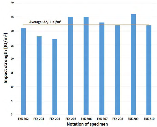
Figure 8. The average of the impact strength values
