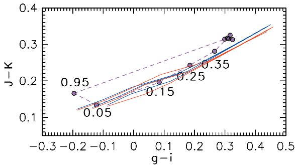
Figure 8. Symbols connected by dashed lines show 2MASS J-K color vs. SDSS g-i color for SDSS J015450+001501. Data were binned in 0.1 wide equidistant phase bins, and the bin centers are marked for a few data points (the motion during pulsational cycle is counterclockwise in this diagram). Although both colors are good estimators of the effective temperature, a hysteresis is easily seen (e.g., at g-i = 0 , about 0.05 mag difference in J-K color). Note that both colors are essentially constant for phase bins from 0.45 to 085. The six thin, solid lines are predictions made on the basis of Kurucz static model atmospheres with effective temperatures in the range 6000–7500 K. At the blue end, they bifurcate into the groups of three tracks—they correspond to models with [\text{Fe}/\text{H}] = -1.5 (the top three curves) and [\text{Fe}/\text{H}] = -1.0 . For each metallicity, the three curves correspond to \log(g) = 2.5, 3.0 and 3.5 . Note that at the blue end, the models bifurcate according to \log(g) , rather than [\text{Fe}/\text{H}] (at J-K \sim 0.13 , the g-i color becomes bluer by \sim 0.1 mag as \log(g) increases from 2.5 to 3.5).
