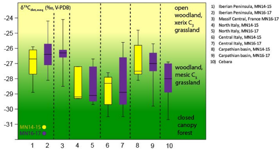
Fig. 3. \delta^{13}\text{C}_{\text{diet,meq}} values in different regions and biozones. The modern equivalent vegetation was calculated using the equations of Kohn (2010). The scale was calculated with Pliocene \delta^{13}\text{C} values of atmospheric \text{CO}_2 . Using a scale for the Early Pleistocene would shift the \delta^{13}\text{C}_{\text{diet,meq}} values by +0.2\% .
