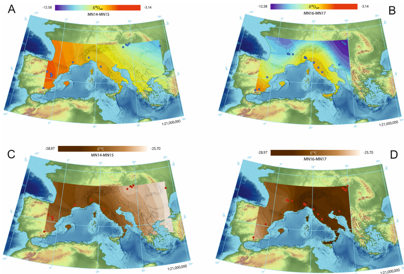
Fig. 2. Color-interpolated maps of the calculated \delta^{18}\text{O}_{\text{ppt}}(\text{‰}, \text{VSMOW}) and calculated average \delta^{13}\text{C}_{\text{diet,meq}}(\text{‰}, \text{VPDB}) values in MN14-MN15 (A and C) and in MN16-17 (B and D) biozones. \delta^{18}\text{O}_{\text{ppt}} scale was calculated using the equation of Kohn and Cerling (2002), \delta^{13}\text{C}_{\text{diet,meq}} was calculated using the equations of Passey et al. (2005) and Kohn (2010). A 5 Ma paleoDEM (Scotese and Wright, 2018) and rotation and geometry files for movement vectors (PaleoAtlas V3, Scotese, 2016) were used as major data sources for the reconstructed map. (For interpretation of the references to colour in this figure legend, the reader is referred to the Web version of this article.)
