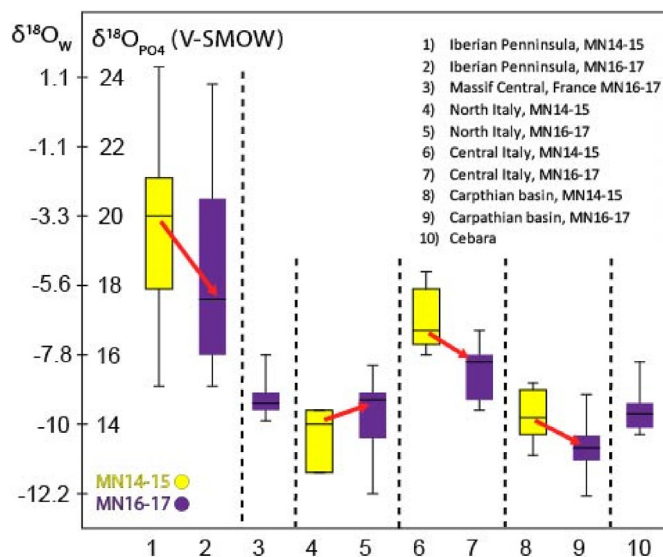
Fig. 4. \delta^{18}\text{O}_w (‰, V-SMOW) values in different regions and biozones. The \delta^{18}\text{O}_w scale was calculated using the equation of Kohn and Cerling (2002).
