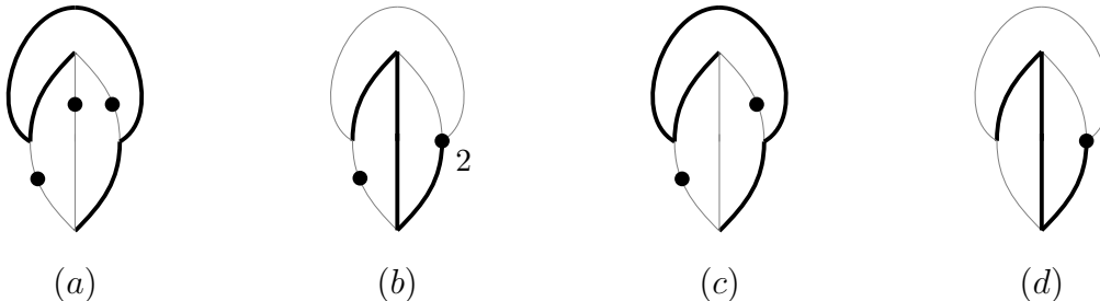
FIGURE 1. Semibreak divisors on a metric graph of genus 3.
