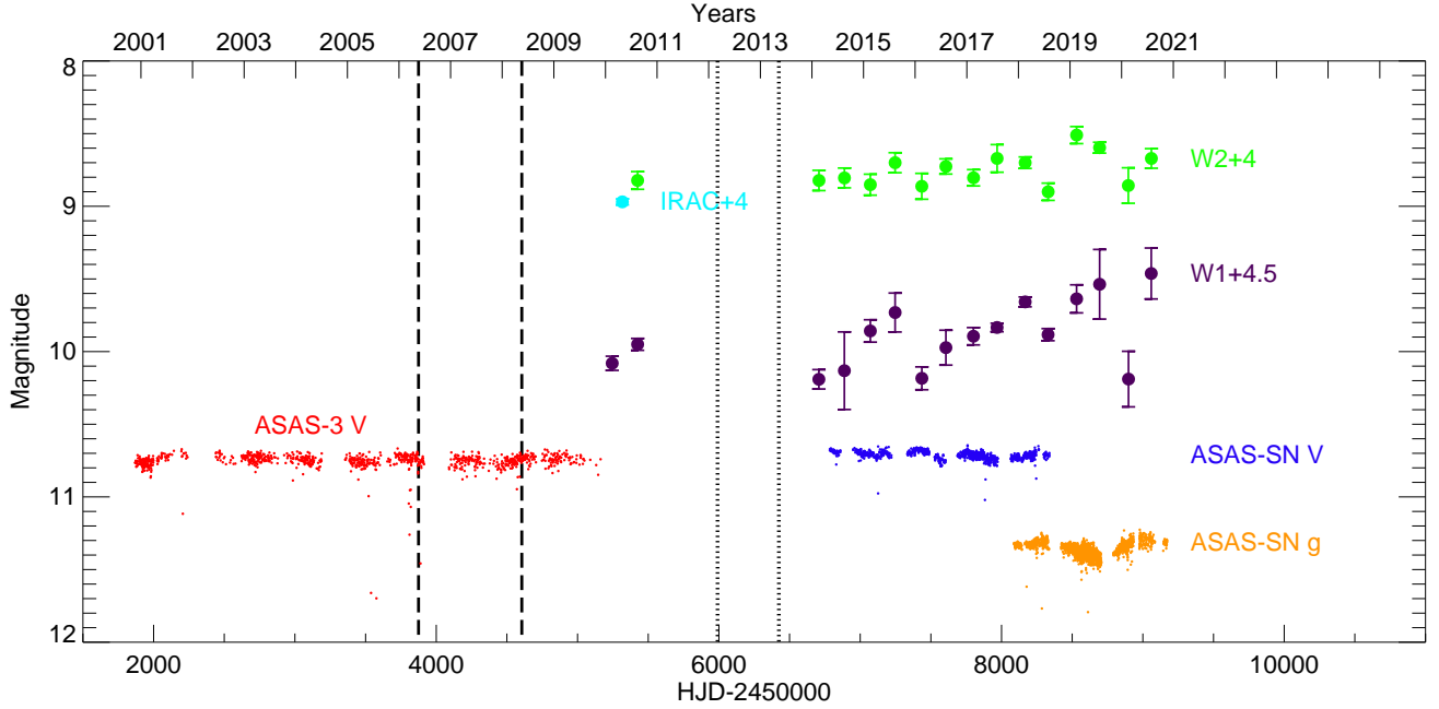
Figure 6. The ASAS and WISE light curves of DI Cha. The vertical dashed lines indicate the epochs of the first and last MIDI observations. The dotted line is same to the PIONIER observations.
