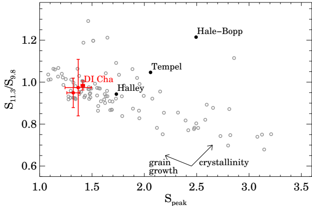
Figure 16. Ratio of the continuum subtracted and normalized 11.3/9.8 \mu\text{m} flux ratio versus the feature strength. DI Cha is marked with red dots. Gray circles mark T Tauri and Herbig Ae/Be stars. Black dots show solar system comets.
