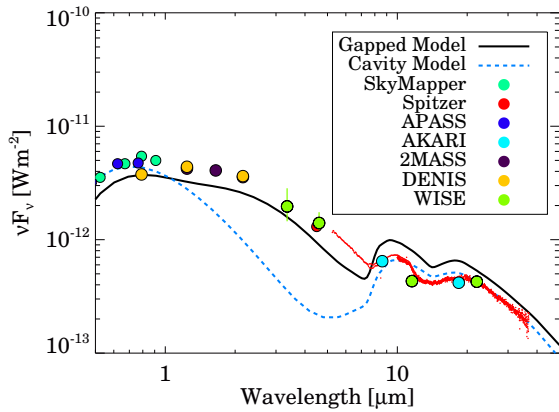
Figure 13. The spectrum of DI Cha. Black curve: SED of the two component model (with gap). Blue dashed curve: SED of the one component (cavity) model.
