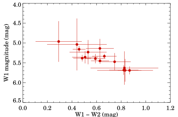
Figure 17. Color-magnitude diagram of the WISE observations.
