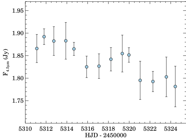
Figure 5. IRAC light curve of DI Cha.
