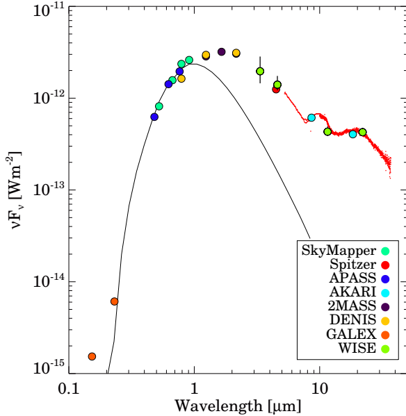
Figure 8. The observed SED of DI Cha. The photometric data came from the following public archives: Spitzer; Luhman et al. (2008), WISE; Cutri & et al. (2012), AKARI; Ishihara et al. (2010), 2MASS; Cutri et al. (2003), Gaia; Gaia Collaboration et al. (2018), SkyMapper; Wolf et al. (2018), DENIS; Denis (2005), APASS; Henden et al. (2018), GALEX; Bianchi et al. (2011). The vertical bar connecting the extreme values of the WISE light curves are plotted to illustrate the variability.
