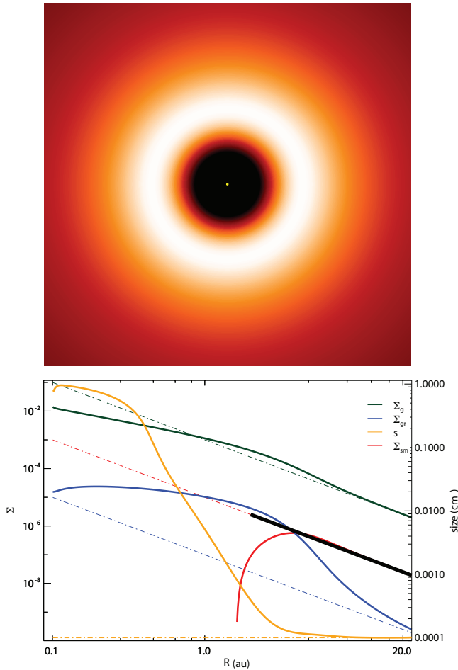
Figure 18. Snapshot of the hydrodynamic simulation that models the two component dust growth. Upper panel: Surface mass density distribution of the small-sized dust component in the inner ( R < 8\text{au} ) disk. Lower panel: Radial profiles of gas (green) and the two dusty components (small-sized (red) and grown dust (blue)). Dot-dashed curves show the initial profiles. Orange line shows the representative particle size of grown dust. Note that the black lines represents the simple radiative transfer model of dusty component.
