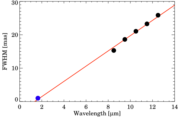
Figure 11. Results of the Gaussian model fitting for each wavelength ranges. The black points marks the MIDI fitting results, the blue point marks the PIONIER fitting result.
