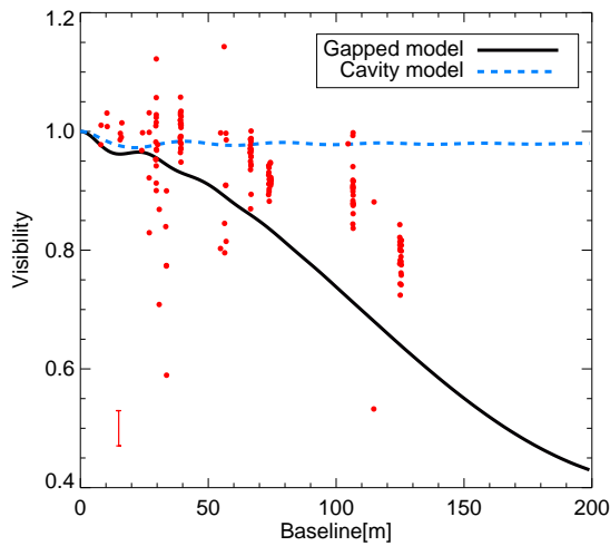
Figure 15. The visibility functions of both models in the H band ( 1.65 \mu\text{m} ), compared with the PIONIER data (red dots). The error bar in the left corner reflects the average dispersion of the data. For the gapped model fitting \chi^2=2.66 and for the cavity model fitting \chi^2=2.44 .
