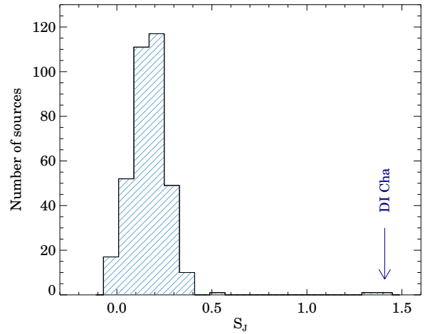
Figure 7. Histogram of the Stetson J variability index, based on 357 reference stars. The S_J value for DI Cha is marked by a blue arrow.
