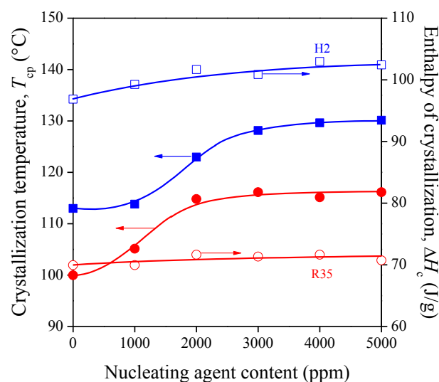
Fig. 1 Crystallization characteristics of PP polymers plotted against the amount of sorbitol clarifier. Effect of polymer characteristics. Symbols: (○,●) random copolymer (R35), (□, ■) homopolymer (H2), (○,□) enthalpy of crystallization, (●,■) peak temperature of crystallization.
