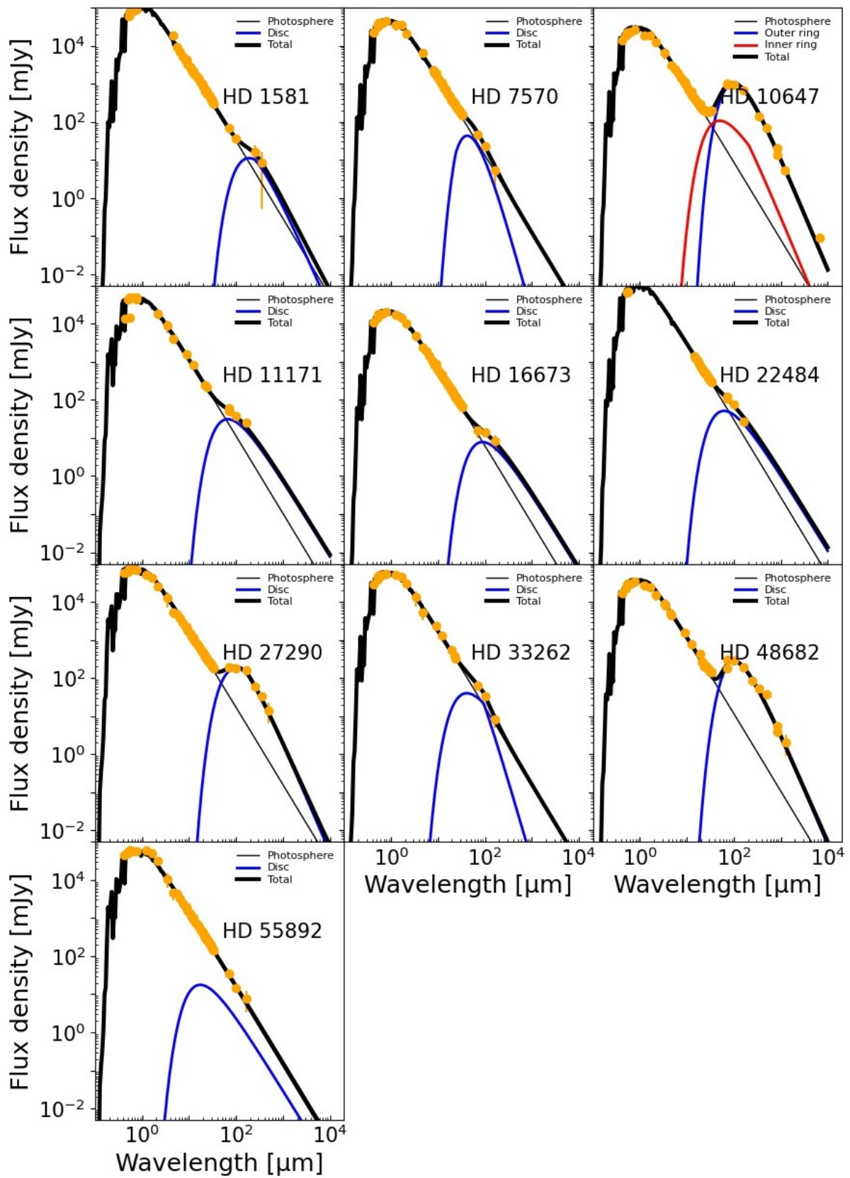
Figure A3. SEDs for the debris discs detected around F stars in the DEBRIS sample.
