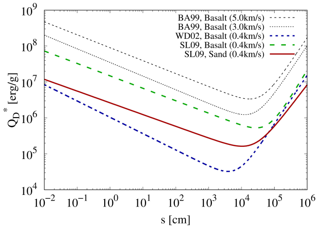
Figure B1. Q_D^* as function of size. The thin black dashed and dotted lines show values for basalt at 3 and 5 km/s taken from Benz & Asphaug (1999). The parameters of the HD 109085 system are assumed. The thick blue dash-dotted line shows the scaling result taken for Wyatt & Dent (2002) and the thick green dashed line the lab results taken from Stewart & Leinhardt (2009) for basalt at 0.4 km/s. The thick solid red line shows the result for “sand” at 0.4 km/s taken from Stewart & Leinhardt (2009).
