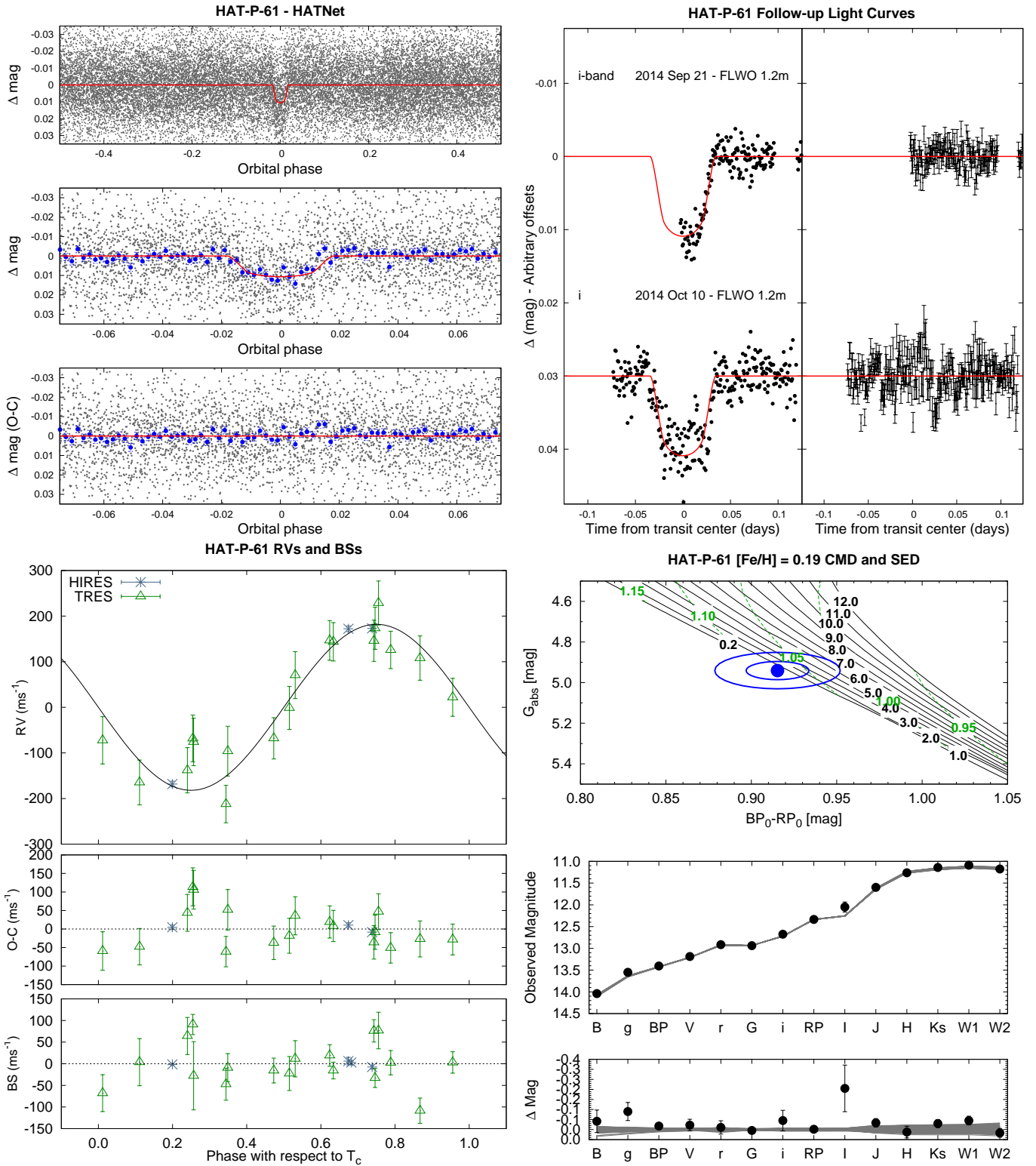
Figure 7. Observations of HAT-P-61 together with our best-fit model. Please refer to Figure 1 for a more detailed caption. The TESS light curve for this system is shown in Figure 13.
