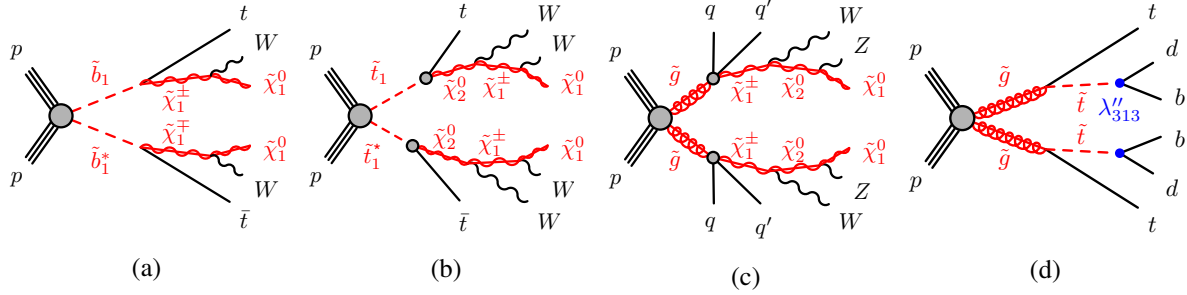
Figure 1: Examples of processes allowed in the MSSM, involving the pair production and cascade decays of squarks and gluinos into final states with leptons and jets.
