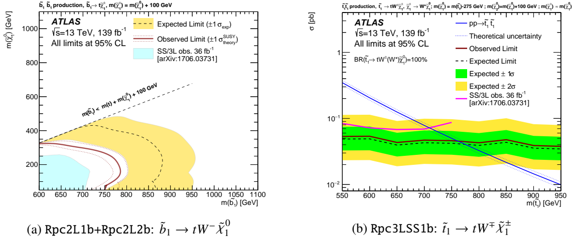
Figure 8: 95% CL exclusion limits on the production of pairs of third-generation squarks, assuming production cross-sections as in Ref. [27] (for the left plot) and 100% branching ratios into the decay modes illustrated in Figures 1(a) and 1(b) for the left and right plots, respectively. The limits are determined from the expected contributions of these processes to the Rpc2L1b and Rpc2L2b (left) and Rpc3LSS1b (right) SRs. The coloured bands display the \pm 1\sigma ranges (as well as \pm 2\sigma for the right figure) of the expected fluctuations around the mean expected limit, in the absence of contributions from the sought-for signals. They do not account for uncertainties in the signal process cross-sections, the impact of which is illustrated by the dashed lines around the observed limits. The figures show for reference the reach of the previous analysis [28].
