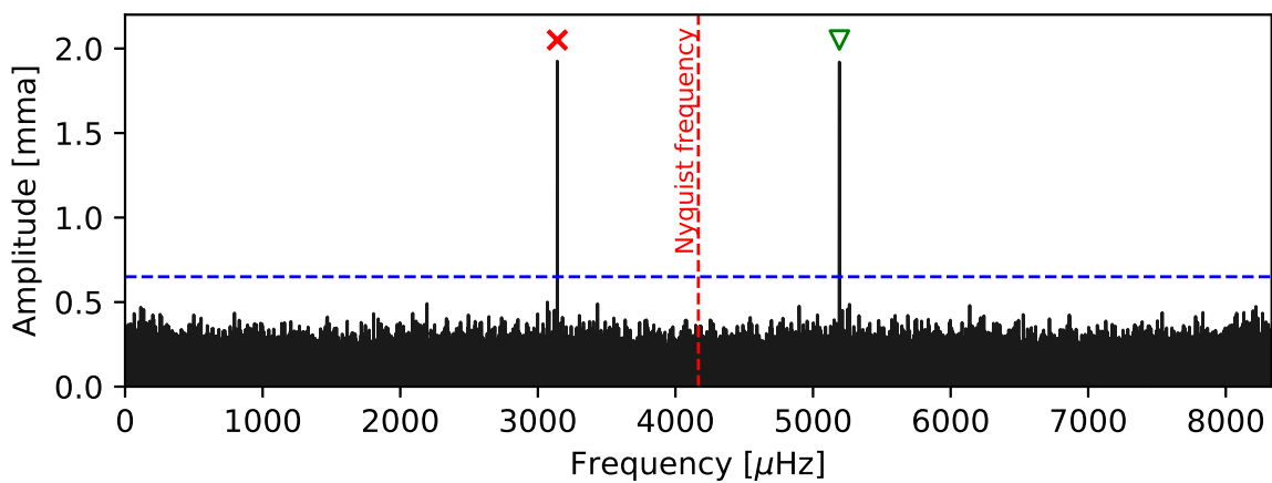
Fig. 9. Fourier transform of the TESS light curve of L 19-2 calculated out to twice the Nyquist frequency. The single significant observed signal is reflected across the Nyquist frequency (red dashed line), with the incorrect sub-Nyquist alias marked with a red \times and the signal at the intrinsic frequency marked with a green triangle. The blue dashed line indicates the 0.1% FAP level.
