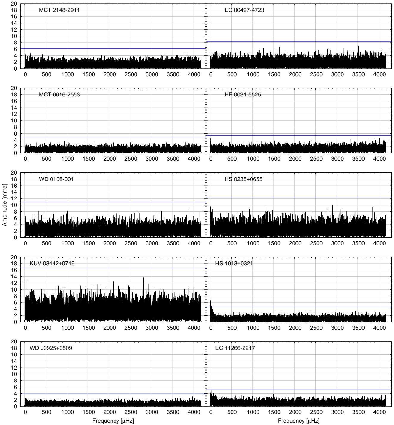
Fig. B.2. Fourier transforms of the ZZ Ceti stars not observed to vary by the TESS data. Blue lines denote the 0.1% FAP levels.
