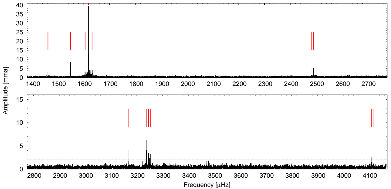
Fig. 4. Fourier transform of the light curve of BPM 31594. Red lines mark the frequencies listed in Table 6, while the blue dashed line represents the 0.1% FAP level ( S/N=4.85 ) calculated by this Fourier transform.
