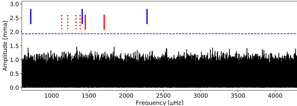
Fig. 10. Fourier transform of Sectors 1–13 of the TESS light curve of HE 0532-5605; the blue dashed line indicates the 0.1% FAP level ( S/N = 5.24 ). Vertical red lines mark the frequencies from Fontaine et al. (2003), dashed lines are additional frequencies from that data reported by Castanheira & Kepler (2009), and blue vertical lines (offset upwards) mark those from Kilkenney et al. (2014).
