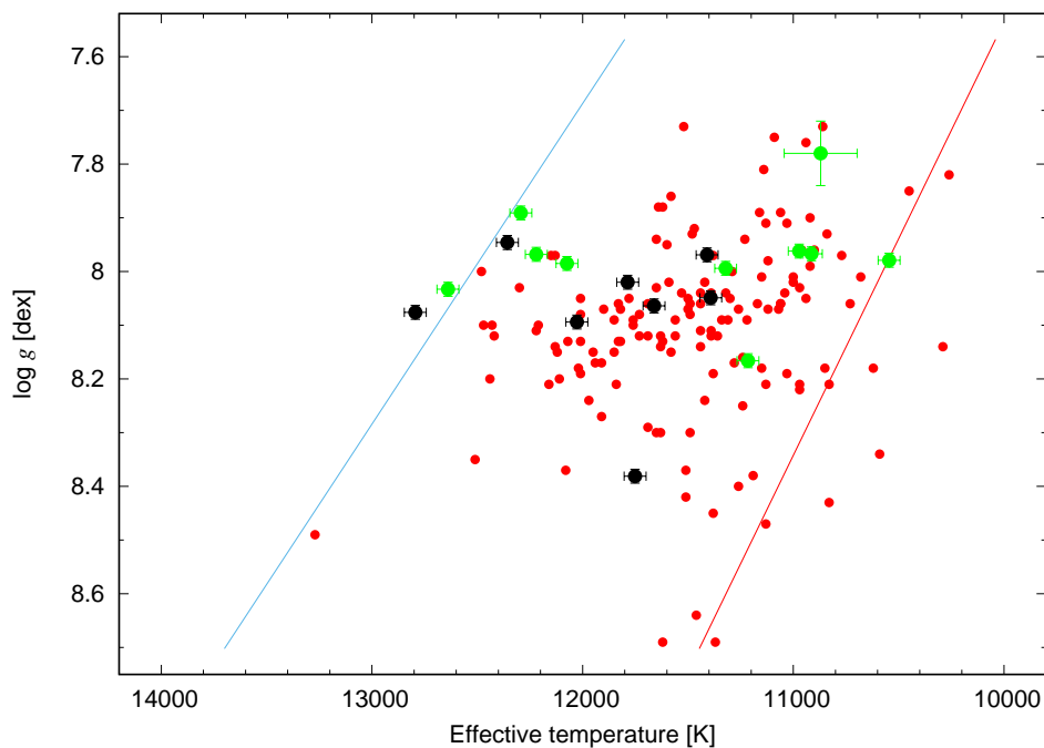
Fig. 15. Known ZZ Ceti stars (red filled dots, atmospheric parameters from Bognár & Sódor 2016), and the DAVs observed by TESS during the survey measurements of the southern ecliptic hemisphere (sectors 1–13) in the T_{\text{eff}} - \log g diagram. Black and green dots mark the stars found to be variable and not observed to vary by the TESS measurements, respectively. Their atmospheric parameters were derived by Fuchs (2017), except in the case of KUV 03442+0719, where we used the values presented in Bognár & Sódor (2016). Blue and red lines denote the hot and cool boundaries of the instability strip, according to Tremblay et al. (2015).
