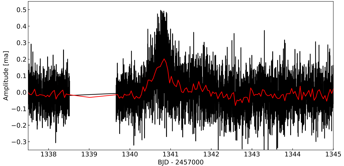
Fig. 12. Light curve of a portion of the Sector 1 observations of HE 0532-5605. The red line is binned light curve, with a bin size of 30 points, to show the amplitude and duration of an apparent brightening of 20% for 24 hours.
