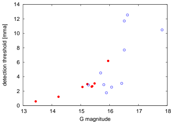
Fig. 16. Pulsation-detection performance of TESS . Stars confirmed (red dots) or not observed to vary (blue circles) by the TESS observations in the G magnitude – detection threshold diagram, where the detection threshold is defined as 0.1\% \text{FAP} \times \sqrt{\text{CROWDSAP}} \times \sqrt{\text{number of sectors}} .
