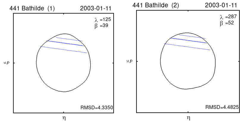
Fig. C.10. Shape model fitting to stellar occultations by 441 Bathilde.
