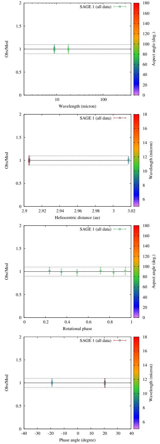
Fig. B.5. (14) Irene (from top to bottom): observation-to-model ratios versus wavelength, heliocentric distance, rotational phase, and phase angle. The plots that correspond to the pole 2 solution are very similar.
