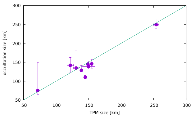
Fig. 7. Set of average occultation diameters vs. diameters from TPM. The straight line is y=x .
