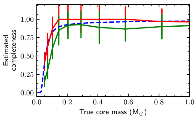
Fig. B.1. Completeness curves for our Herschel census of candidate prestellar cores based on Monte-Carlo simulations using a population of synthetic prestellar cores detected by getsources and classified as candidate prestellar cores (green solid curve) or classified as (bound or unbound) starless cores (red solid curve). For comparison, the dashed blue curve shows the completeness curve predicted by the simple model of the core extraction process described in Appendix B.2 of Könyves et al. (2015), scaled to the distance of the Ophiuchus cloud ( d = 139 pc).
