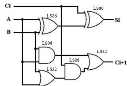
Figure 3 Full adder
