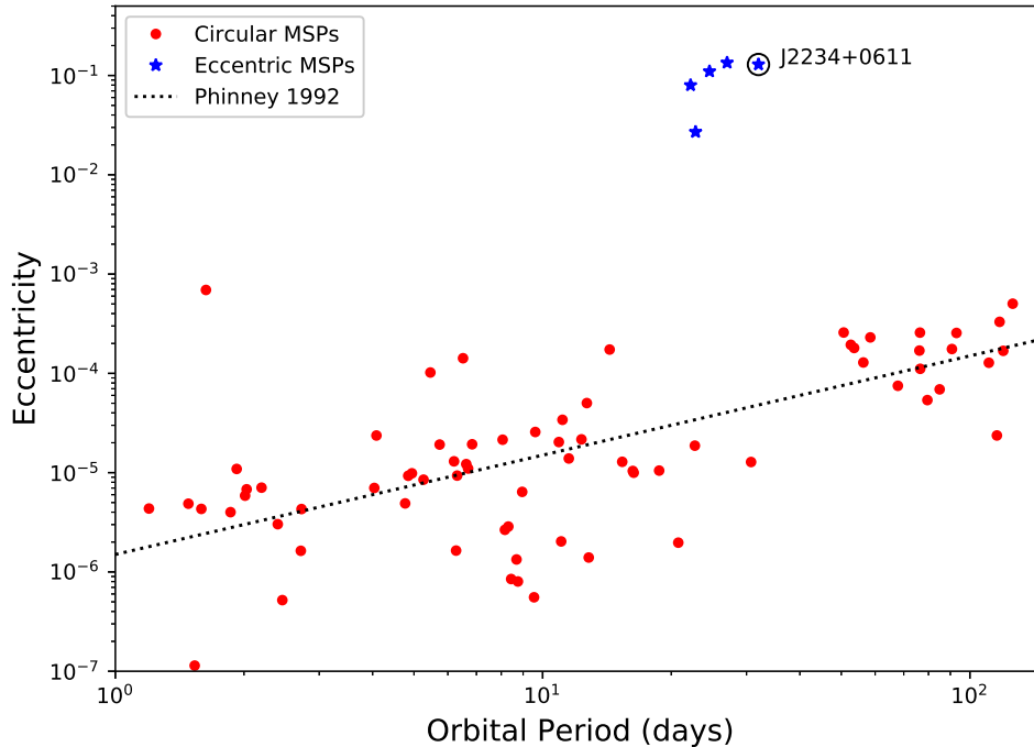
Figure 1. Eccentricity ( e ) versus orbital period ( P_b ) for recycled pulsars with low-mass ( < 0.6M_\odot ) companions outside globular clusters. The eccentric MSPs, blue stars, stand out from the general MSP population, red circles. For the latter, the orbital eccentricities are small and generally follow the evolution predicted by Phinney (1992), shown by the black dotted line. Note that there is an under-density of circular MSP systems within the orbital period range where the eccentric MSPs are found and going to larger orbital periods, as first noted by (Camilo 1995).
