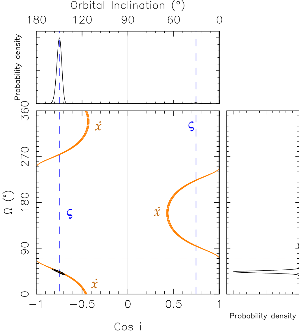
Figure 5. Orbital orientation constraints for PSR J2234+0611. In the main square panel we display the full \cos i - \Omega plane; this has a priori a constant probability density for randomly aligned systems. The black contours include 68.23 and 95.44% of the total probability density function (pdf) derived from a 3-dimensional \chi^2 map of \cos i - \Omega - M_{\text{tot}} space using the DDK model with the additional assumption that GR is the correct theory of gravity. The dashed orange line indicates the PA of the proper motion of the system ( \Theta_\mu = 69.0(1) deg). The dashed blue line indicates the \zeta assumed in our DDFWHE model; the solid orange lines indicate the regions that are consistent with the nominal and \pm 1-\sigma measurements of \dot{x} obtained in that model (see Table 2). The \zeta and \dot{x} constraints predict well the location of the region(s) of high probability but provide no distinction between the four locations where they cross (these are listed in Table 3); this can only be done using the DDK model (see text for details). The side panels display the 1-d pdfs for \cos i (top) and \Omega (right).
