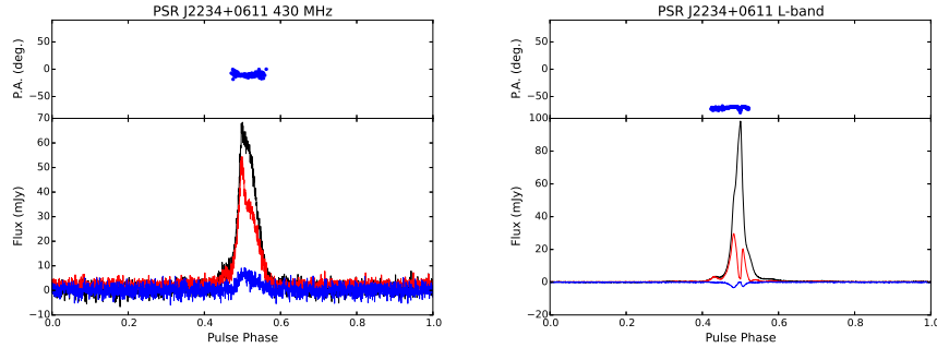
Figure 2. Polarimetric profiles for PSR J2234+0611 at 430 MHz (left) and 1.5 GHz (right) from the Arecibo Observatory using the PUPPI backend with bandwidths of 20 and 650 MHz, respectively. These profiles were taken from individual high signal-to-noise ratio detections. The top panels show the polarization angle versus pulse phase. The bottom panels show the total intensity (black), linear polarization (red), and circular polarization (blue) versus pulse phase. The profiles have been polarization and flux calibrated using the methods described in Arzoumanian et al. (2018). These profiles have not been corrected for rotation measure, as the value measured from these observations is consistent with 0 \text{ rad m}^{-2} . Additional analysis of the polarization properties for PSR J2234+0611 has been presented in Gentile et al. (2018).
