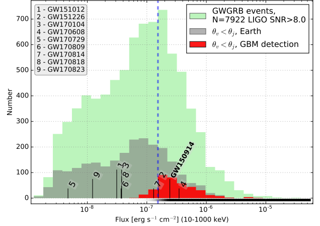
Figure 4. Expected gamma-ray flux distribution from BBH, arising in the charged BH scenario (Section 3.3). Note that in this case we present GW signals with SNR>8. The BBH-to-GRB ratio (ratio of numbers in the green to red histogram) is 7922/381 = 20.8. This is the expected number of BBH mergers GBM has to follow until the detection of the next gamma-ray counterpart. Notations are similar to Figure 2.
