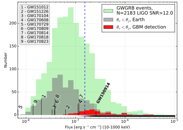
Figure 5. Example of observed sources, where the EM energy is a fraction \epsilon_{GW} = 3.4 \times 10^{-6} \text{ s}^{-1} of the emitted GW radiation ( L_\gamma = \epsilon_{GW} E_{GW} , Section 3.4). In the above example the BBH-to-GRB ratio is 34.1. Notations are similar to Figure 2
