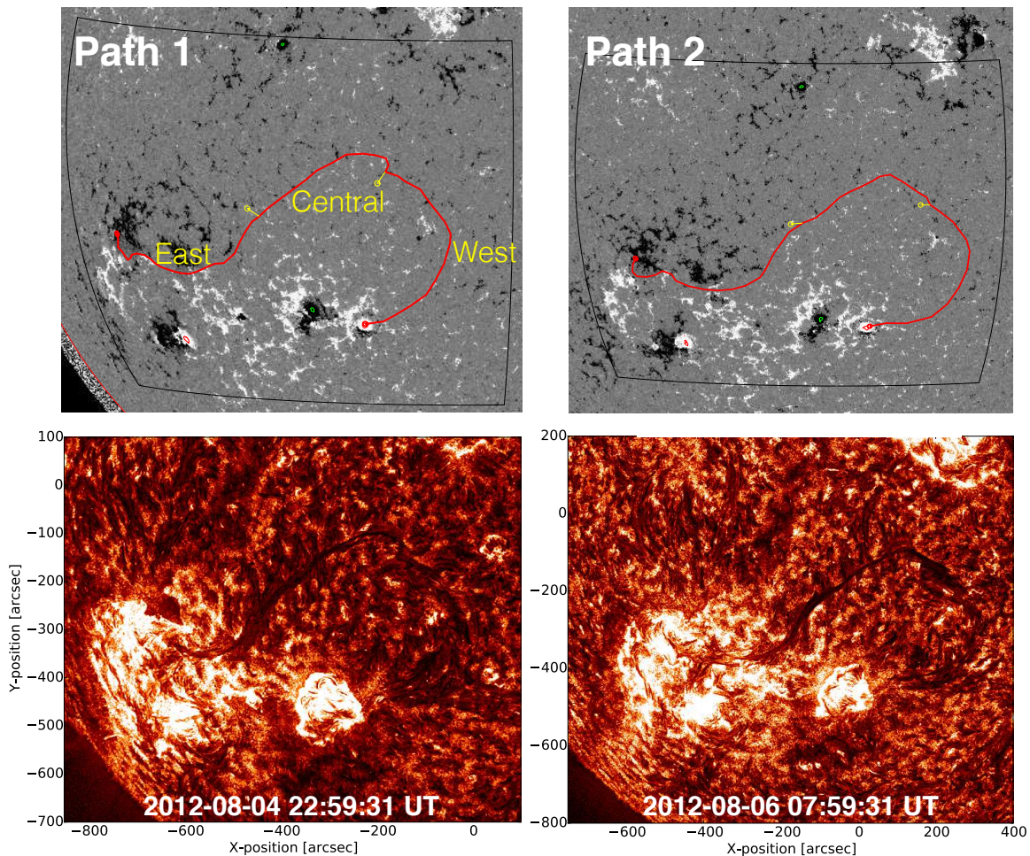
Figure 5. SDO/HMI magnetograms and the corresponding SDO/AIA 304 Å images of the filament taken around the times of the two magnetic models (2012 August 4 23:00 UT and August 6 08:00 UT). The magnetograms have a saturation of \pm 100 G and the 304 Å images have been enhanced using the MGN technique. The red curves represent the path along which the flux rope is inserted into the model. The path is divided into three sections: east, central and west as determined by the locations of the two main barbs of the filament (yellow bars in the top panel). The first section is at the eastern end where the flux rope is rooted in the negative polarity of AR 11541, the middle section is between the two barbs and the final section is between the second barb and the end rooted in the positive polarity of AR 11538. Each section has a different value of axial flux, which is given in Table 1.
