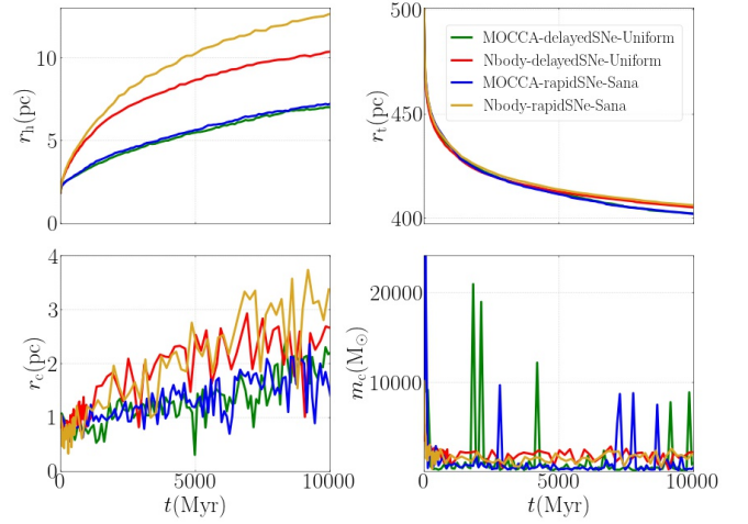
Figure 1. Time evolution of the half-mass radii r_h (pc) (top-left), the tidal radii r_t (pc) (top-right), core radii r_c (pc) (bottom-left) and core masses m_c ( M_{\odot} ) (bottom-right) for the four simulations. The Nbody-delayedSNe-Uniform, Nbody-rapidSNe-Sana, MOCCA-delayedSNe-Uniform and MOCCA-rapidSNe-Sana simulations are shown in red, yellow, green and blue, respectively.
