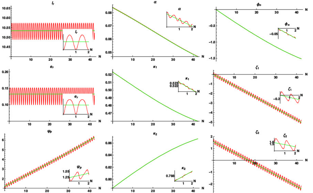
Figure 1: The panels represent the secular (green) and instantaneous (red) evolutions of l_r , e_r , \alpha , \phi_n , \psi_p , \kappa_i and \zeta_i ( i = 1, 2 ) as functions of the number of orbital periods N . The parameters and initial conditions for the instantaneous evolutions are: total mass m = 20M_\odot , mass ratio \nu = 0.5 , dimensionless spin parameters \chi_1 = \chi_2 = 0.9982 , eccentricity e_r(0) = 0.1 , spin polar angles \kappa_1(0) = \pi/6 and \kappa_2(0) = \pi/4 , spin azimuthal angles \zeta_1(0) = 0 and \zeta_2(0) = \pi/2 , longitude of the ascending node \phi_n(0) = 0 and post-Newtonian parameter \varepsilon(0) = 0.01 . Matching initial conditions for the secular dynamics have been chosen, as explained in the main text. On some of the plots the two evolutions overlap at the chosen resolution. On each panel the first two periods are also shown in order to illustrate that the match only occurs on the longer run.
