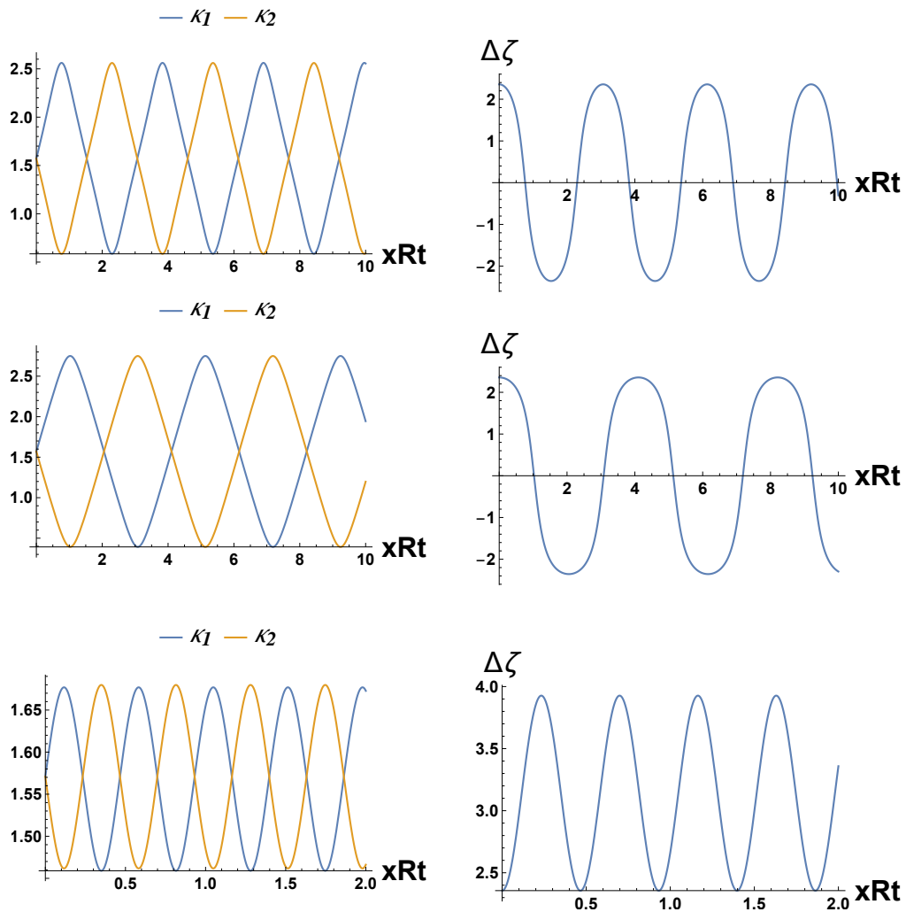
Figure 6: The evolution of the spin polar angles (left column) and of the difference of their azimuthal angle (right column) as function of the dimensionless time t in units of xR , for binaries consisting of a black hole and either a gravastar with w = -0.8 (first row), another black hole (second row) or a boson star with w = 100 (third row). The mass ratio is \nu = 1 in all cases. The plots are for the PN parameter \bar{\varepsilon} = 0.0001 , eccentricity \bar{e}_r = 0.1 , the parameters x \equiv x_1 = x_2 = 0.01 , and initial spin orientations \kappa_1(0) = \kappa_2(0) = \pi/2 , \Delta\zeta(0) = 3\pi/4 . The polar angles exhibit a flip-flopping behavior, with both the frequency and amplitude depending on the quadrupole parameter of the compact companion. The difference of the azimuthal angles is also sensitive to w .
