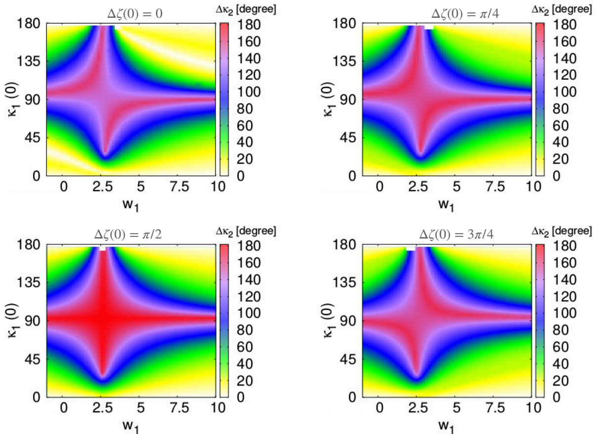
Figure 5: The color map represents the flip-flop angle \Delta\kappa_2 as a function of the initial polar angle \kappa_1(0) and the quadrupole parameter w_1 of the dominant spin ( \chi_1 \gg \chi_2 ). From the top left to lower right panel, \Delta\zeta(0) is 0 , \pi/4 , \pi/2 , and 3\pi/4 , respectively. The additional parameters of the binary are m_1 = m_2 = 1.4M_\odot , \bar{e}_r = 0.1 , \bar{\varepsilon} = 0.0001 , \chi_1 = 0.95 , \chi_2 = 0.05 , and \kappa_2(0) = \pi/10 . In the small white rectangle regions, \Delta\kappa_2 does not reach its maximum within the conservative timescale. The flip-flop is large in the red diamond-shaped regions.
