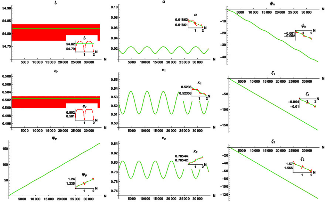
Figure 4: The effect of an increased eccentricity e_r(0) = 0.5 , the rest of the parameters being identical to those for Fig. 3.
