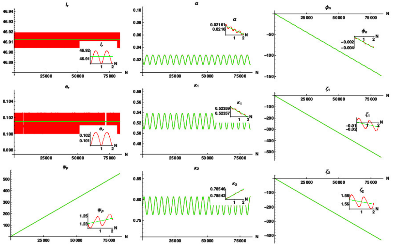
Figure 3: The evolutions at a much earlier stage of the inspiral, characterized by post-Newtonian parameter \varepsilon(0) = 0.0005 , the rest of the parameters being identical to those for Fig. 1.
