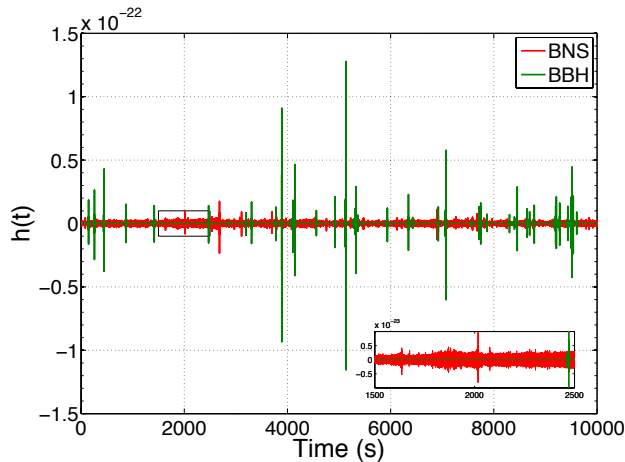
FIG. 2. We present a simulated time series of duration 10^4 seconds illustrating the character of the BBH and BNS signals in the time domain. In red we show a simulated BNS background corresponding to the median rate as shown in Figure 1, and in green we display the median BBH background. We do not show any detector noise, and do not remove some loud and close events that would be detected individually. The region in the black box, from 1800 – 2600 seconds, is shown in greater detail in the inset. The BNS time series is continuous as it consists of a superposition of overlapping signals. On the other hand the BBH background (in green) is popcorn-like, and the signals do not overlap. Remarkably, even though the backgrounds have very different structure in the time domain, the energy in both backgrounds are comparable below 100 Hz, as seen in Figure 1.
