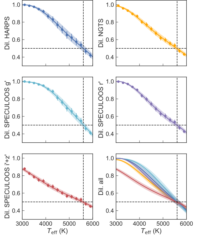
Figure 8. HARPS, NGTS and SPECULOOS dilution of star B, D_{0,B} , as function of its effective temperature of NGTS-3B, T_{\text{eff},B} . We derive the dilution by passing PHOENIX model spectra through the telescope bandpasses. We fit the resulting trend with a 5th-order polynomial, which can then be used to predict the dilution for each instrument at any chosen T_{\text{eff},B} . Dashed lines at dilution 0.5 and T_{\text{eff}} \approx 5600 K indicate the properties of star A. Note that, when modelling a planet on star A, the dilution of the planet signal on star A is calculated as D_{0,A} = 1 - D_{0,B} .
