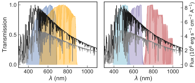
Figure 7. Dilution is a function of the instrument transmission and stellar spectral types. Left axis: Transmission efficiency of HARPS (blue), NGTS (orange) and the SPECULOOS g' -band (light blue), r' -band (purple), and i'+z' -band (red), all including atmospheric absorption. Right axis: luminosity of a G6V (top) and a K4V (bottom) star. The different bandpasses lead to a different dilution of the planetary signal for each instrument.
