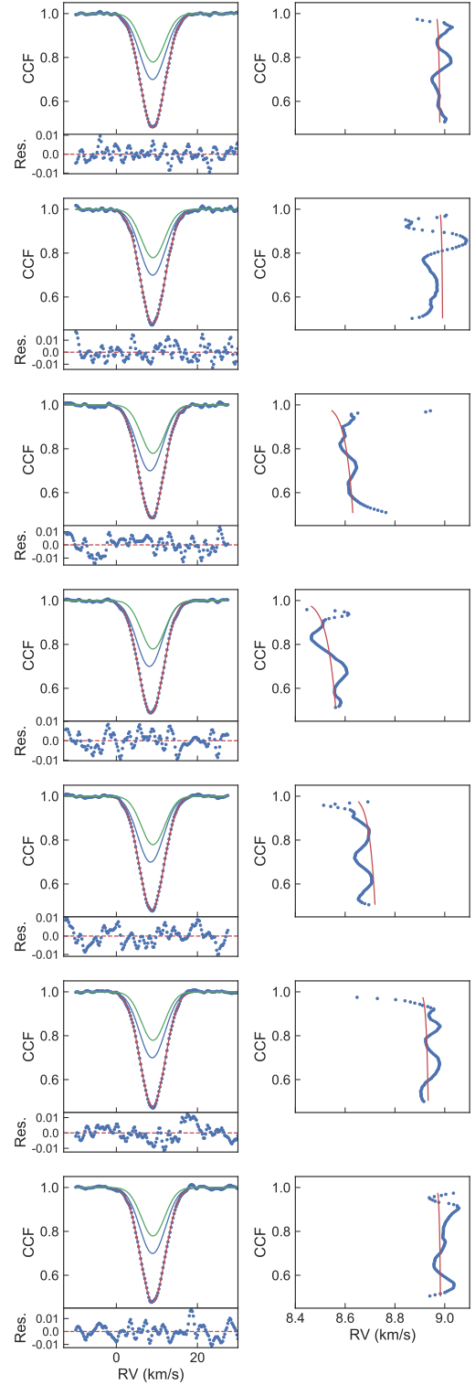
Figure 3. The seven HARPS CCF profiles (left column), and zoom onto their extracted bisectors (right column). Left column: the shown CCF profiles are corrected for the best-fit baseline from the global BLENDFITTER MCMC model. Red lines show the MCMC results for the best fit of the movement of two stars, modelled as two Gaussian profiles. The model for star A is shown in green, star B in blue and their sum in red. Sub-panels show the residuals of the fit. Right column: bisectors were extracted by BLENDFITTER using the second derivatives of the Gaussian fit.
