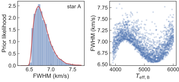
Figure 6. Prior likelihood distributions for the FWHM of star A (A) and star B (B), the latter expressed as a function of T_{\text{eff},B} . Note the minima of the FWHM relation for early K-type stars.
