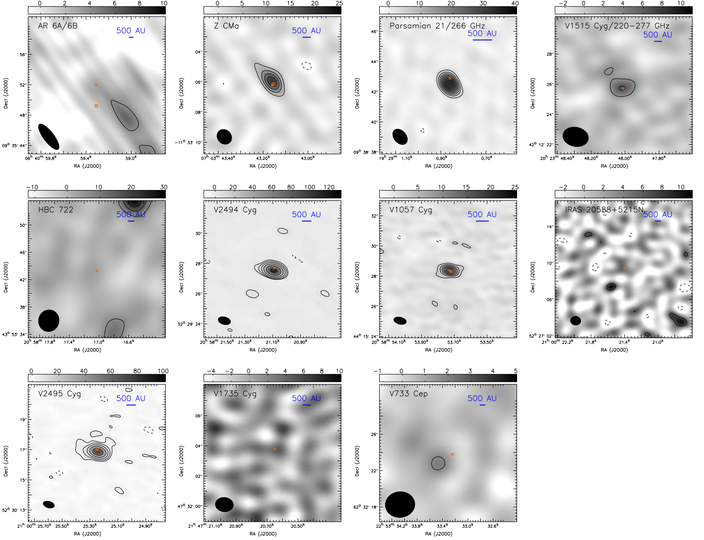
Fig. 2. Continuation of Figure 1. Contours of V2494 Cyg are 1.0 \text{ mJy beam}^{-1} ( 1\sigma ) \times [-3, 3, 6, 12, 24, 48, 96]. Rectangle and cross in the panel of AR 6A/6B marks the locations of AR 6A and 6B quoted from Aspin & Reipurth (2003); those in the panel of Z CMa mark the locations of Z CMa NW and SE, respectively (Szeifert et al. 2010).
