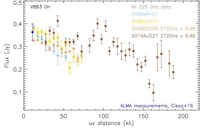
Fig. 9. Visibility amplitudes of V883 Ori (similar to Figure 7). We scaled the observed amplitudes at frequencies higher than 225 GHz to the expected amplitudes at this frequency, by assuming the spectral index \alpha = 4.0 . We overplot the integrated flux measured at the same frequency by ALMA with 11 k\lambda shortest uv distance, which were taken on December 12 of 2014 and April 05 of 2015 (Cieza et al. 2016). We assume a nominal 10% error bar for the presented ALMA measurement. There were ALMA observations taken with the more extended array configuration in August and October of 2015. We omit presenting measurements from the extended ALMA array observations since they observed quasars as absolute flux references, which are not ideal for the purpose of studying flux variability.
