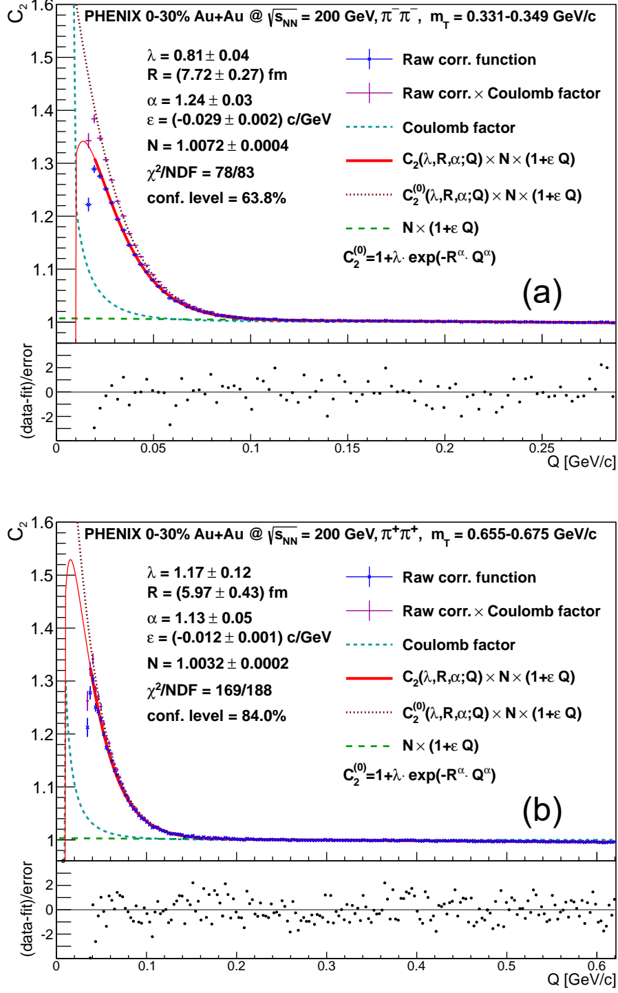
FIG. 3. Example fits of Bose-Einstein correlation functions of (a) \pi^- \pi^- pair with m_T between 0.331 and 0.349 GeV/c 2 and of (b) \pi^+ \pi^+ pair with m_T between 0.655 and 0.675 GeV/c 2 , as a function Q \equiv |\mathbf{q}_{LCMS}| , defined in Eq. (26). Both fits show the measured correlation function and the complete fit function (described in VIA), while a Bose-Einstein fit function C_2^{(0)}(Q) is also shown, with the Coulomb-corrected data, i.e. the raw data multiplied by C_2^{(0)}(Q)/C_2(Q) . In this analysis we measured 62 such correlation functions (for ++ and -- pairs, in 31 m_T bins), and fitted all of them with the method described in VIA. The first visible point on both panels corresponds to Q values below the accessible range (based on an evaluation of the two-track cuts), these were not taken into account in the fitting.
