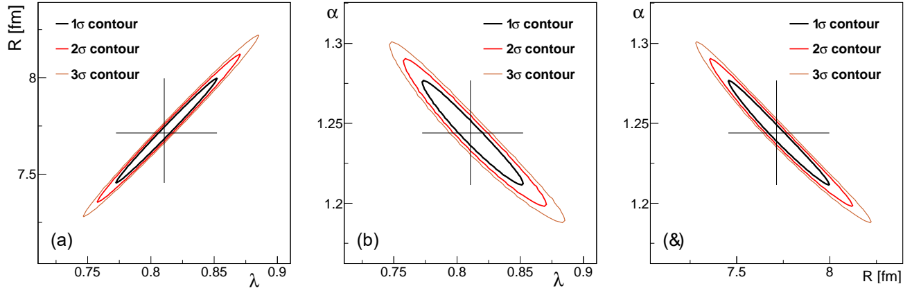
FIG. 7. Contour lines of the \chi^2 map in the (a) \lambda, R and (b) \lambda, \alpha and (c) R, \alpha planes for fits to \pi^-\pi^- correlation functions of pairs with m_T between 0.331 and 0.349 \text{GeV}/c^2 . The horizontal and vertical lines represent the MINOS fit uncertainties.
