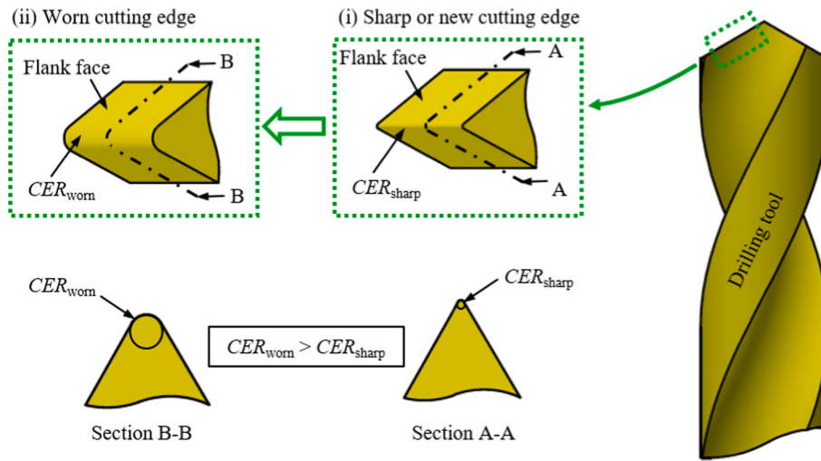
Fig. 15. Cutting-edge rounding (CER): (a) sharp cutting edge; (b) rounded cutting edge (redrawn based on Ref. [47]).
