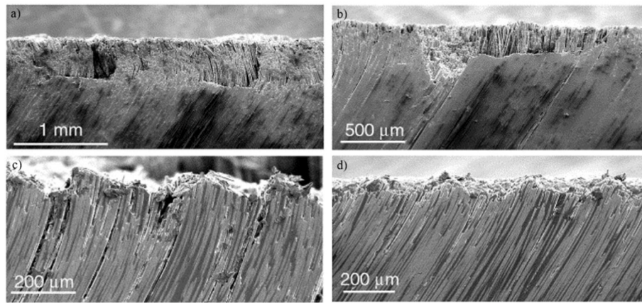
Fig. 12. Subsurface microstructure at fibre orientation of 120°, depth of cut of 0.1 mm and rake angle of [104] (a) -20^\circ , (b) 0^\circ , (c) 20^\circ , (d) 40^\circ .
