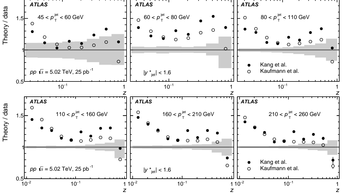
Figure 9: Ratios of theoretical calculations from Refs. [50, 51] (solid points) and Ref. [52] (open points) to the unfolded pp D(z) distributions for the six p_T^{\text{jet}} intervals used in this analysis. The statistical uncertainties are shown as error bars and the systematic uncertainties in the data are shown as the shaded region around unity. The uncertainties in the theoretical calculations are not shown.
