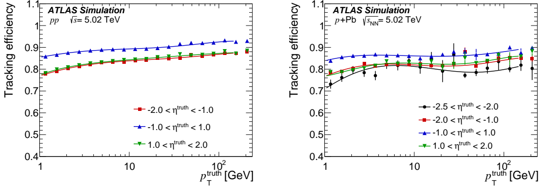
Figure 1: Tracking efficiency as a function the primary particle momentum at generation level, p_T^{\text{truth}} , in pp collisions (left) and in p +Pb collisions for one of the two beam configurations (right). The different sets of points show the primary particle pseudorapidity, \eta^{\text{truth}} , intervals in which the track reconstruction efficiency has been performed. The different \eta^{\text{truth}} intervals in pp and p +Pb plots reflect the different regions of the tracking system used in the two cases due to the boosted p +Pb system. The solid curves show parameterizations of efficiencies.
