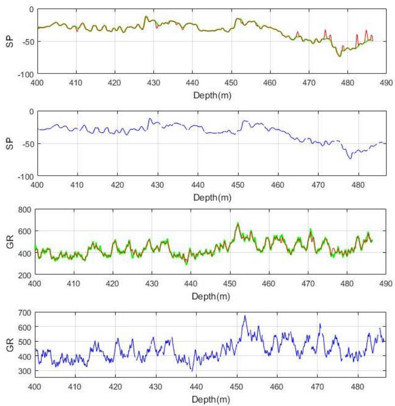
Figure 2. Measured (green) and estimated (red) sections in terms of depth (from left to right: E40, SP, GR, GG, NN, CAL) for 10% missing values
