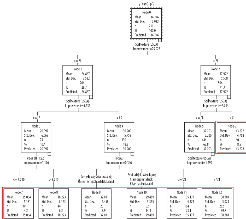
Fig. 3. Water content estimation, an example for pF = 2, classes definition based on soil main type, soil reaction (pH water) and texture class (USDA). M = predicted mean value of the node; STD = standard deviation; n = number of samples, % = percentage of samples used at the node; I = improvement; SL = sandy loam; LS = loamy sand; CL = clay loam; SCL = sandy clay loam. The relation signs in context of the USDA texture classes can be interpreted by the following sequence built in the model: 1 = sand; 2 = loamy sand; 3 = sandy loam; 4 = loam; 5 = sandy clay loam; 6 = sandy clay; 7 = silty clay; 8 = silt; 9 = silty clay loam; 10 = clay loam; 11 = silty clay; 12 = clay.
