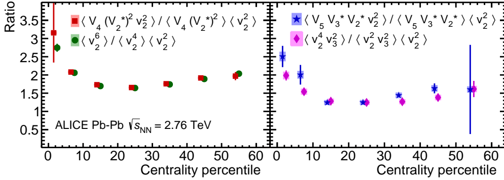
Fig. 1: Study of relationship between linear and non-linear modes in higher order anisotropic flow in Pb–Pb collisions at \sqrt{s_{\text{NN}}} = 2.76 TeV, according to Eqs. (7) and (8).
