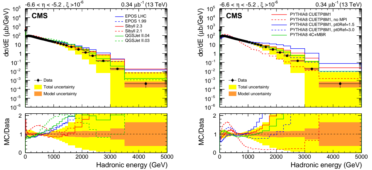
Figure 5: Differential cross section as a function of the hadronic energy in the region -6.6 < \eta < -5.2 for events with \xi > 10^{-6} . The left panel shows the data compared to MC event generators mostly developed for cosmic ray induced air showers, and the right panel to different PYTHIA 8 tunes.
