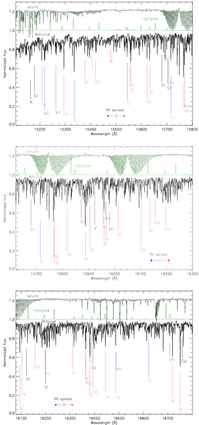
FIG. 2.— In three overlapping wavelength regions, the distribution of telluric absorption ( top spectra in each panel ), airglow ( middle spectra ), and atomic lines in the spectrum of the star Arcturus ( bottom spectra ). Some prominent atomic lines in the Arcturus spectrum that guided the ultimate selection of the APOGEE wavelength region are identified and color-coded as high priority ( red ), medium priority ( blue ) and lower priority ( black ). Also indicated are the extremes in the potential shift in the lines from extremes in radial velocity variation for potential (e.g., halo) Milky Way stars (adopted as \pm 700 \text{ km s}^{-1} in the lines).
