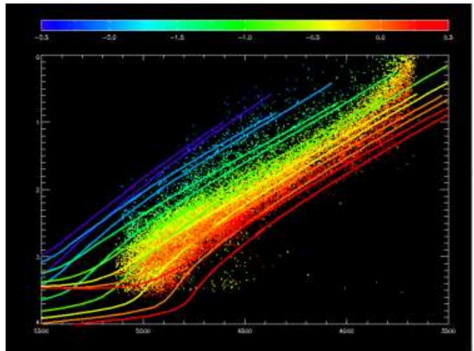
FIG. 20.— Final, calibrated, ASPCAP-derived parameters for main survey stars in the nominal temperature range of the APOGEE main sample. Colors show the metallicities derived for the stars according to the scale at the top. The lines show Padova PARSEC (Bressan et al. 2012) isochrones for 4 Gyr populations at various metallicities, against which the calibrated spectral metallicities may be compared.
