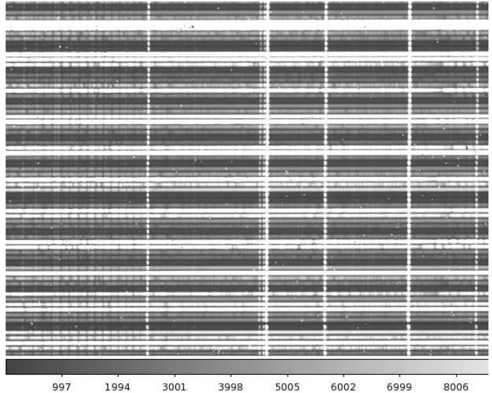
FIG. 14.— A portion of a raw 2-D APOGEE image from observations of a bulge field. The horizontal stripes correspond to individual stellar spectra. Vertical bright bands correspond to airglow features at the same rest wavelength in each spectrum, whereas absorption features at the same horizontal position from spectrum to spectrum correspond to telluric absorption features. Also obvious are variations in the expression of stellar atmospheric absorption features from star to star, evidenced by their varying strengths due to temperature and chemical composition differences, as well as changing relative positions due to Doppler shifts. Fiber assignments were managed by color-coding the fiber jackets at the telescope end for stars in each field sorted into three brightness groups (bright, medium, faint). These fibers were sorted at the spectrograph slit head into a repeating pattern of faint-medium-bright-bright-medium-faint to minimize the contamination of any given spectrum by the PSF wings of a much brighter spectrum in an adjacent fiber. This management scheme gives rise to the brightness modulation pattern apparent in this image.
