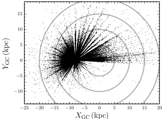
FIG. 16.— The computed Galactic distribution of APOGEE targets as projected on the Galactic plane. Comparison to Figure 11 shows that the anticipated spatial coverage of the Milky Way has been achieved.
