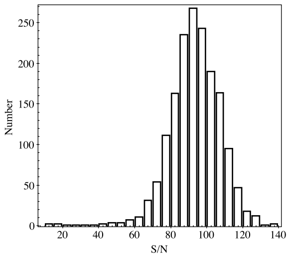
FIG. 19.— Distribution of S/N for stars with 12.15 < H < 12.20 for stars on 3-visit plugplates.
