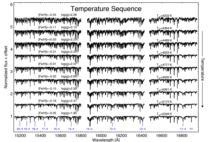
FIG. 7.— An image showing continuum normalized APOGEE spectra as a function of stellar surface temperature for typical APOGEE main survey RGB stars of near-solar abundance. At the bottom, Bracket hydrogen lines are identified; these lines show the clear trend of increasing strength for increasing temperature.
