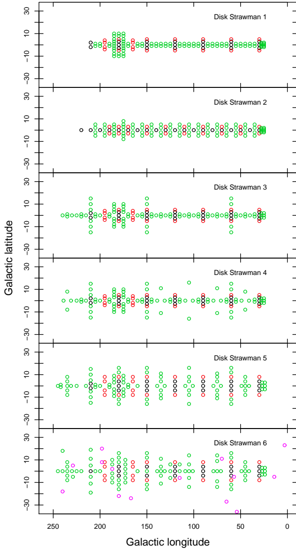
FIG. 36.— Evolution of the design of the disk field distribution is seen from the earliest plan, “Disk Strawman 1”, to the nearly final disk plan, “Disk Strawman 6”. Green circles represent 3-hour fields, red circles are 10- or 12-hour fields, and black circles are 24- or 30-hour fields.
