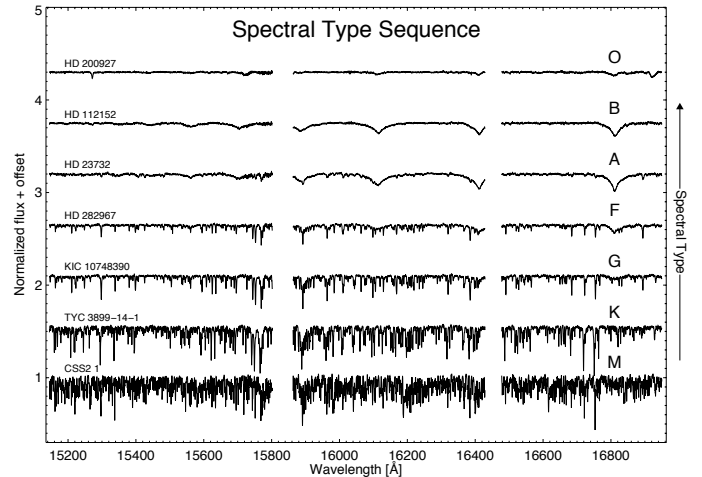
FIG. 6.— An image showing continuum normalized APOGEE spectra as a function of stellar spectral type. The earlier spectral types are representative of those seen among the telluric standards, whereas the later types are typical of those seen among the main APOGEE survey.
