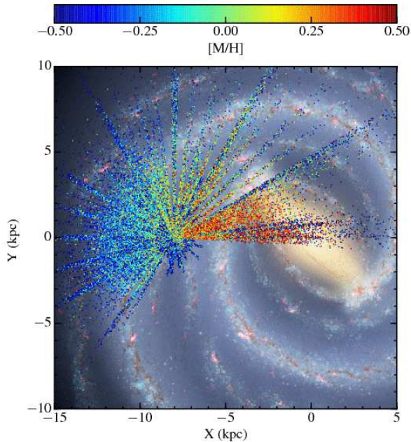
FIG. 25.— Same as Fig. 24, but with points color-coded by metallicities [M/H] and using stars with projected |Z_{GC}| < 2 kpc. (Background image credit, R. Hurt, NASA/JPL-Caltech.)
