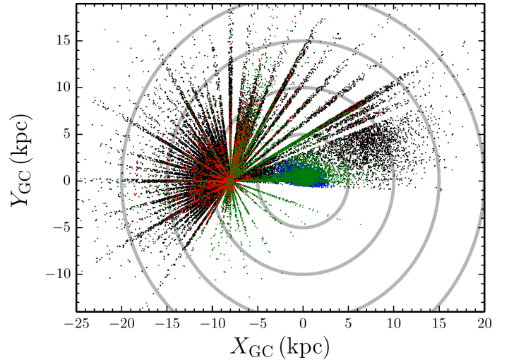
FIG. 11.— The expected Galactic distribution of APOGEE targets as projected on the Galactic plane, as predicted by the Trilegal model for the field plan prior to the final, survey year three modifications. Stars are color-coded by expected stellar population: blue = bulge, green=halo, red=thick disk, black=thin disk.
