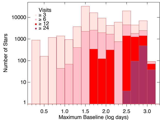
FIG. 18.— ( Top ) Distribution of the number of stars having a given number of visits over the course of the survey. ( Bottom ) Maximum time baseline for stars having at least 3, 6, 12, or 24 visits.
