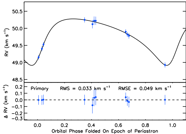
FIG. 23.— (Re-)discovery of the hot Jupiter around HD 114762 using eleven epochs of APOGEE data.
