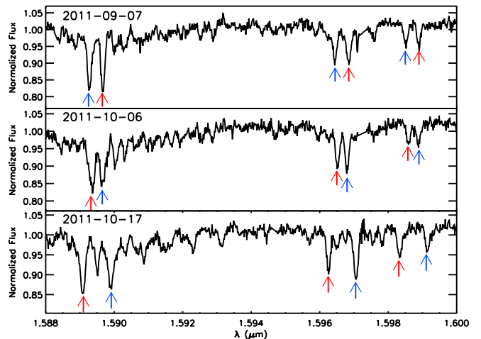
FIG. 21.— Time series data of a double-line spectroscopic binary, illustrating the variation in the position of the lines for both the primary (lines marked by blue arrows) and secondary (red arrows) stars in the system.
