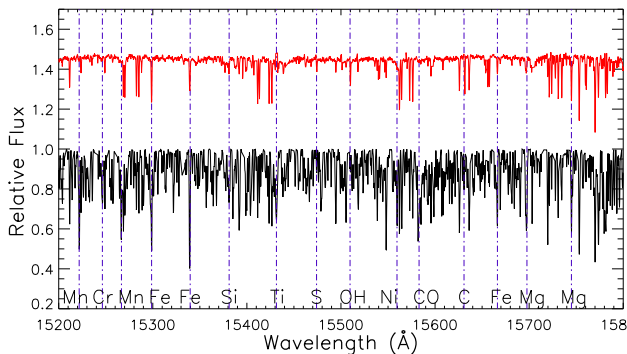
FIG. 9.— Comparison of a section of the APOGEE spectra for two stars of the same temperature (approximately 4060 K) with about a 100\times ratio in abundance of iron. The red spectrum is for a star that has [\text{Fe}/\text{H}] = -1.8 and \log g = 0.158 . The black spectrum is for a star that has [\text{Fe}/\text{H}] = 0.365 and \log g = 1.5 .
