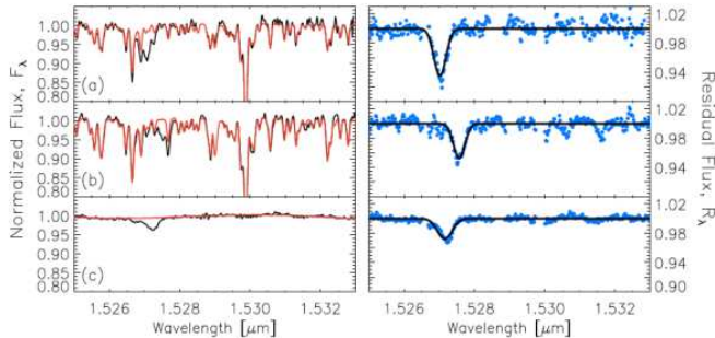
FIG. 32.— (Left) Comparison of synthetic (red lines) to observed APOGEE spectra (black lines) for two late type giant stars (panels a and b) and a hotter star (panel c) star. (Right) The difference spectra (blue points) clearly show the DIB feature at 15,272 Å, which can be fit with simple Gaussians (black lines) to measure column density and varying Doppler velocities (Zasowski et al. 2015).
