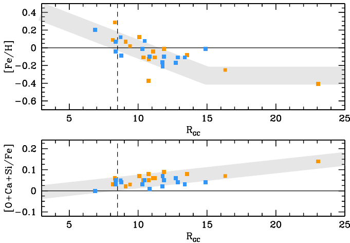
FIG. 29.— APOGEE-derived metallicity and [\alpha/\text{Fe}] (using the reliable individual DR12 elements O+Ca+Si as \alpha ) as a function of Galactocentric radius for 29 clusters in two age regimes: Blue (orange) points denote clusters younger (older) than 1 Gyr. The light grey region in the upper panel shows a gradient in [\text{Fe}/\text{H}] of -0.06 \text{ dex kpc}^{-1} within R_{GC} = 15 \text{ kpc} and hints of a flat distribution (admittedly based on very few data points) beyond with a spread of 0.2 dex. A shallower, positive gradient, of +0.007 \text{ kpc}^{-1} \text{ dex} , is seen in [\alpha/\text{Fe}] (lower panel) consistent with previous literature-based open cluster studies (e.g., Yong et al. 2012). Additional individual element abundance gradients are explored in Frinchaboy et al. (2015).
