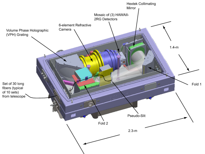
FIG. 4.— Layout of the APOGEE spectrograph optical bench within the cryostat. The fiber train coming from the telescope enters the cryostat on the left.
