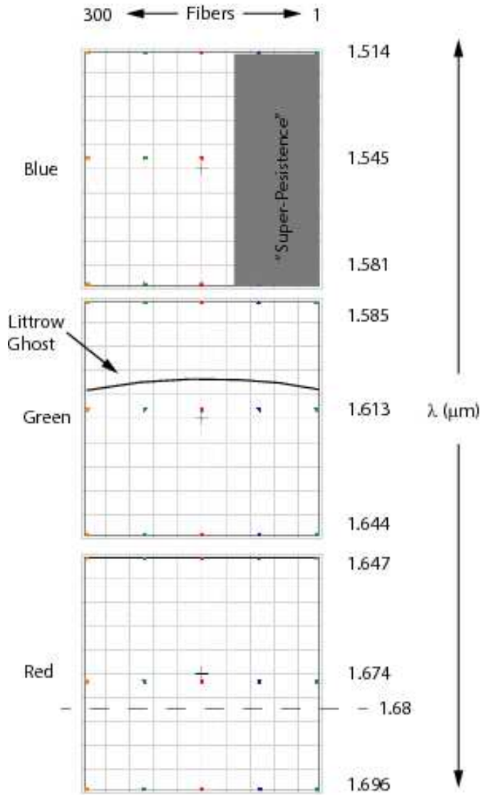
FIG. 5.— Schematic figure showing the arrangement of fibers and wavelengths across the three APOGEE detectors. The wavelengths indicate the edges of the arrays as well as fiducial wavelength positions (indicated by grey dots) corresponding to the “mid-chip” properties given in Table 2. The location of the Littrow ghost (curved line) and the super-persistent region (grey area) are also indicated. The dashed line at 1.68 \mu\text{m} shows the red limit of the wavelength coverage for which the technical performance of the instrument was specified by the science requirements, but the instrument performance is still good redward of this.
