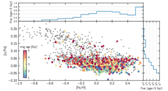
FIG. 28.— Chemical abundance patterns informed by individual stellar ages, derived from the combination of Kepler astroseismology and APOGEE chemistry (see Martig et al. 2015).
