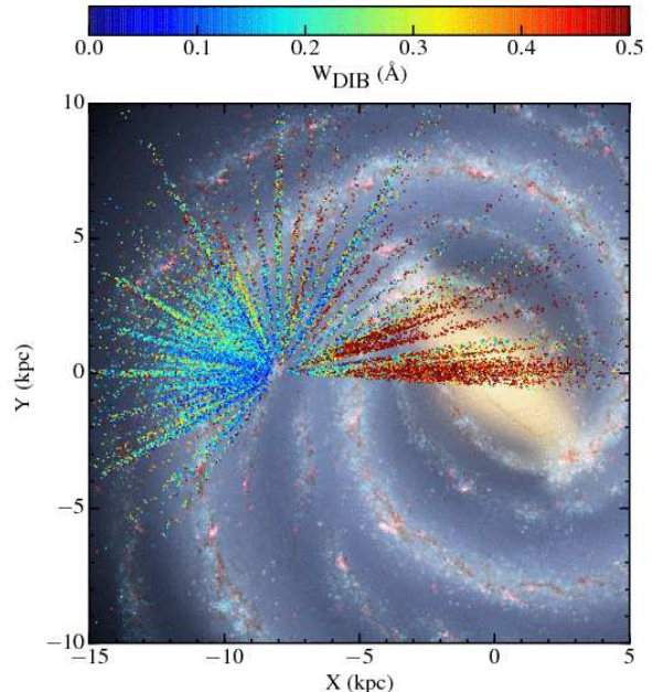
FIG. 33.— Same as Fig. 31, but for the distribution of measured \lambda 15,272 Å DIB strength (Zasowski et al. 2015). As with Fig. 31, the plotted points correspond to the projected locations of the stars against which the DIB absorption was observed. Only stars from DR12 having |Z_{GC}| < 500 pc are shown. (Background image credit, R. Hurt, NASA/JPL-Caltech.)
