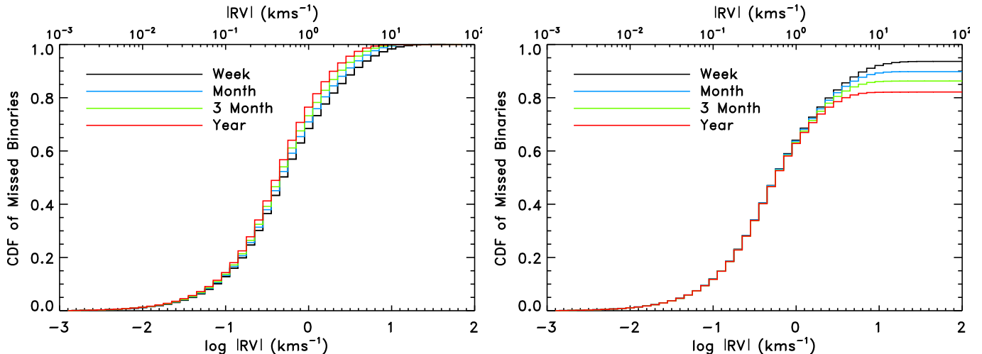
FIG. 35.— Normalized cumulative distribution functions of the fraction of stars having a given APOGEE-measured radial velocity offset from the true systemic velocity for the four different observing cadences described in the text. Note that these are shown only for the binaries that are not flagged as a “likely binary” using the >4 \text{ km s}^{-1} pairwise-difference criterion described in §2.8. In the lefthand plots the normalizations are to the total number of binaries missed for that cadence. In the righthand plot, the distributions are normalized to the total number of simulated binaries; thus, the difference in the maximum CDF-value between each cadence corresponds to the different fractions of “missed binaries”.
