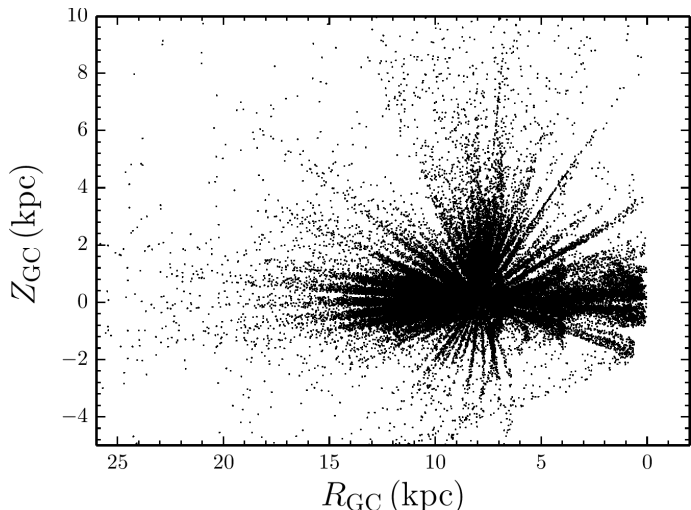
FIG. 17.— Same as Fig. 16 for the computed azimuthally-averaged R_{GC} - Z_{GC} distribution of main APOGEE survey targets. Compare to pre-survey prediction in Fig.12.
