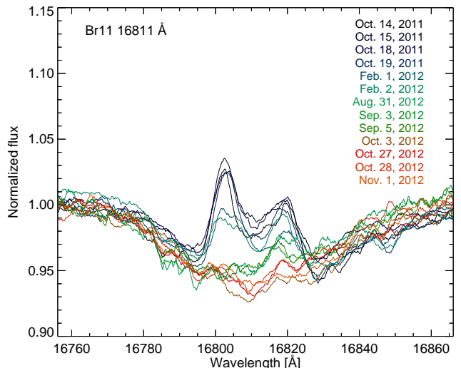
FIG. 22.— Close-up view of the variation in the Brackett 11 (16811 Å) line in one of the Be stars discovered by APOGEE (HD 232940, with V = 9.45 , H = 8.62 ).
