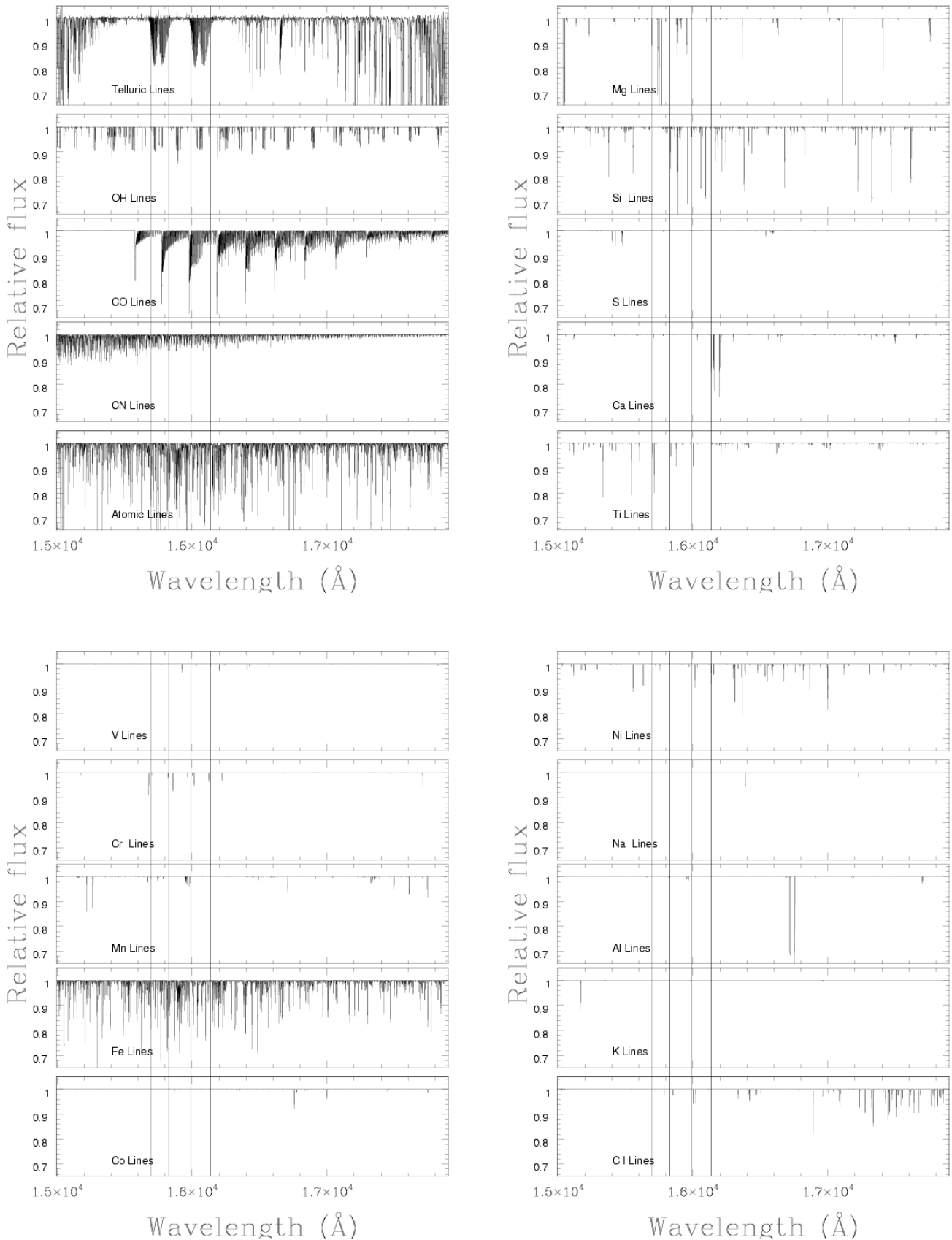
FIG. 34.— Line maps of specific molecules and elements having lines/bands expressed in the H -band. Generally, these are C, N, O, Na, Mg, Al, Si, S, K, Ca, Ti, V, Cr, Mn, Fe, Co and Ni. This is a useful subset of elements with which to probe most types of nucleosynthesis and chemical evolutions. The vertical lines in each plot indicate the ranges of the strong telluric absorption features near 1.6 \mu\text{m} .
