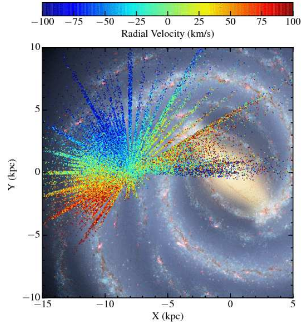
FIG. 24.— Star-by-star APOGEE heliocentric velocities as a function of Galactic X - Y position and projected on an artist’s conception image of the Milky Way. The points represent main APOGEE survey stars (i.e., excluding those in the Kepler field) having projected |Z_{GC}| < 2 \text{ kpc} and \log g \geq 1 . Only stars with no “bad” flags in the database are used. (Background image credit, R. Hurt, NASA/JPL-Caltech.)
