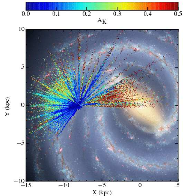
FIG. 31.— Distribution of extinction across the Galactic plane, as measured by comparing star-by-star photometric and spectroscopic data to derive A_{K_s} , according to the isochrone matching method discussed in Schultheis et al. (2014). Point positions correspond to the projected locations of the stars against which the extinction was measured. Only stars from DR12 with |Z_{GC}| < 500 \text{ pc} are shown. Note the substantial increase in extinction at the spiral arm towards the outer disk and also towards the Galactic center. (Background image credit, R. Hurt, NASA/JPL-Caltech.)
