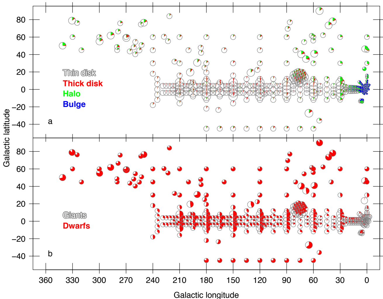
FIG. 38.— Example of Trilegal modeling of the expected distributions of of different properties of sampled stars. Each field position is represented by a pie chart describing target distributions of Galactic component membership (panel a) and evolutionary stage (panel b). In both panels, symbol size is proportional to number of visits. (a) Expected distributions of stars from each of the major Galactic stellar populations on a field-by-field basis. This same distribution is shown in an alternative, Cartesian format in Figures 11 and 12. According to the simulation, thin disk (bulge) fields would be expected to be dominated by thin disk (bulge) stars. However, in halo fields the modeled contribution by thin disk stars is overestimated in this particular simulation, for several reasons. Many halo fields were placed on known overdensities (which increases the relative halo contribution) and globular clusters, where targets were selected to maximize cluster membership; these strategies are not taken into account in the Trilegal simulation, which is based on a Galactic model composed of symmetrical thin and thick disks, halo, and bulge. Moreover, the simulation does not include the effect of the additional halo field selection criterion based on Washington+DDO photometry (§4.2.2), which was designed to minimize (predominantly disk) dwarf contamination, and, indeed, was motivated by model results like that shown here. (b) Example of Trilegal modeling of the expected giant/dwarf ratio on a field-by-field basis, for the final, approved APOGEE plan (after MARVELS descope). This model shows that the disk fields were expected to be dominated by giants (as borne out by the survey); on the other hand, the modeled dwarf/giant ratio in halo fields is much higher than found in the actual survey, because of the additional implemented strategies explained above.
