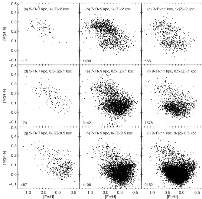
FIG. 27.— Spatial variation of [Mg/Fe] vs. [Fe/H] distributions across the Galactic disk, from Nidever et al. (2014)
