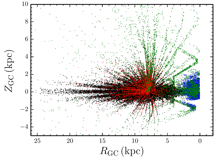
FIG. 12.— Same as above Fig. 11 for the expected Galactic azimuthally-averaged R_{GC}-Z_{GC} distribution of APOGEE targets as predicted by the Trilegal model.
