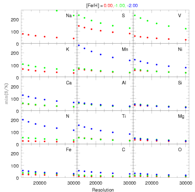
FIG. 3.— Summary of the S/N experiments described in Appendix B for each of 15 chemical elements. For each, the minimum required S/N to measure 0.1 dex precision abundances is plotted for a variety of resolutions from R = 15,000 to 30,000 , and for three metallicities, [\text{Fe}/\text{H}] = -2, -1, \text{ and } 0 . For Al, Si, and Mg the data points for all three modeled metallicities fall on top of one another.
