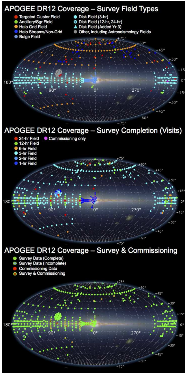
FIG. 10.— (Top) The final APOGEE field targeting plan, the product of the evolving strategy described in §4.1.2. Fields are color-coded by their primary purpose or sought-after target class. The grey fields include both Kepler and CoRoT asteroseismology targets in the Kepler and CoRoT databases, as well as MARVELS Calibration fields. (Middle) Distribution of observed APOGEE fields, color-coded by the number of approximately 1-hour visits. (Bottom) Distribution of APOGEE survey and commissioning fields, and, for the former, whether the survey observations were completed. Most commissioning observations were repeated during the main survey with the spectrograph in its survey configuration.
