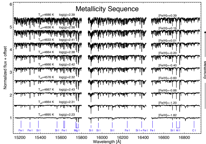
FIG. 8.— An image showing continuum normalized APOGEE spectra as a function of metallicity for giant stars of similar temperature. Some of the strongest metal lines seen are identified at the bottom of the figure.
