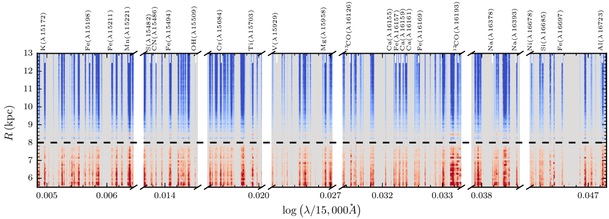
FIG. 26.— Direct spectral representation of the Milky Way disk’s metallicity gradient. This figure displays median-stacked normalized APOGEE spectra of RC stars in bins of Galactocentric radius of width 0.1 kpc and normalized by the spectrum at the solar circle (assumed to be R = 8 kpc, indicated by the dashed line). Redder/bluer colors represent more/less absorption compared to that at the solar circle. Only about 1/6th of the full APOGEE spectral range is shown here, primarily regions containing strong, clean lines and representing all of the elements whose abundances can be determined from APOGEE spectra. Some of the interesting lines of neutral-atomic and molecular species as well as their central wavelengths are labeled at the top. Because RC stars span a narrow range of stellar parameters, absorption line strengths translate into rough elemental abundances directly. All elements display a clear abundance gradient from the inner to the outer disk. The only exception perhaps is vanadium, which is based on a very weak line at 15929Å that becomes vanishingly weak beyond the solar circle.
