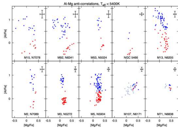
FIG. 30.— Abundance anti-correlations as seen for 428 giant star members in ten Northern Hemisphere globular clusters. Figure from Mészáros et al. (2015).
