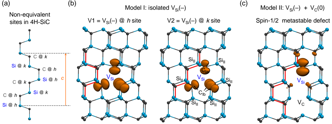
FIG. 1. Models of V1-V2 silicon vacancy related qubits in 4H -SiC. (a) Non-equivalent atomic sites, i.e. a quasi-hexagonal h and a quasi-cubic k sites, in the primitive cell of 4H -SiC. (b) Isolated vacancy model and the assignment of V1-V2 centers to the different silicon vacancy configurations in 4H -SiC. (c) Vacancy pair model of V2 center [14]. In (b) and (c) red lines highlights the stacking of the Si-C double layers to help to identify different configurations of silicon and carbon vacancies. Orange lobes show the spin density of the defects. Based on our first principles results, the isolated vacancy model in (b) can be assigned to V1 and V2 centers in 4H -SiC.
