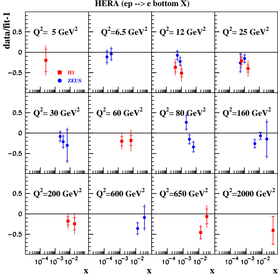
FIG. 15: The same as Fig. 14 for the NC DIS inclusive bottom-quark production data from the H1 [15] (squares) and ZEUS [16] (circles) collaborations at HERA.
