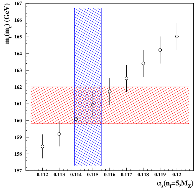
FIG. 31: The \overline{MS} value of the t -quark mass m_t(m_t) obtained in the variants of present analysis with the value of \alpha_s^{(n_f=5)}(M_Z) fixed in comparison with the 1\sigma bands for m_t(m_t) and \alpha_s^{(n_f=5)}(M_Z) obtained in our nominal fit (left-tilted and right-tilted hatch, respectively).
