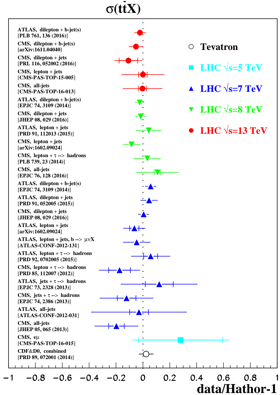
FIG. 16: The pulls for data on top-quark pair production from the Tevatron (CDF and DØ collaborations) at \sqrt{s} = 1.96 TeV and the LHC (ATLAS and CMS collaboration) at \sqrt{s} = 5, 7, 8 and 13 TeV with respect to our NNLO fit. The NNLO QCD predictions have been obtained with Hathor [186].
