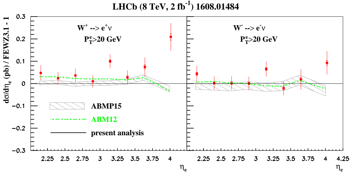
FIG. 11: The same as Fig. 10 for the LHCb data on the cross section of inclusive pp \rightarrow W^+ + X \rightarrow e^+ \nu + X (left) and pp \rightarrow W^- + X \rightarrow e^- \nu + X (right) production at 8 TeV [198].
