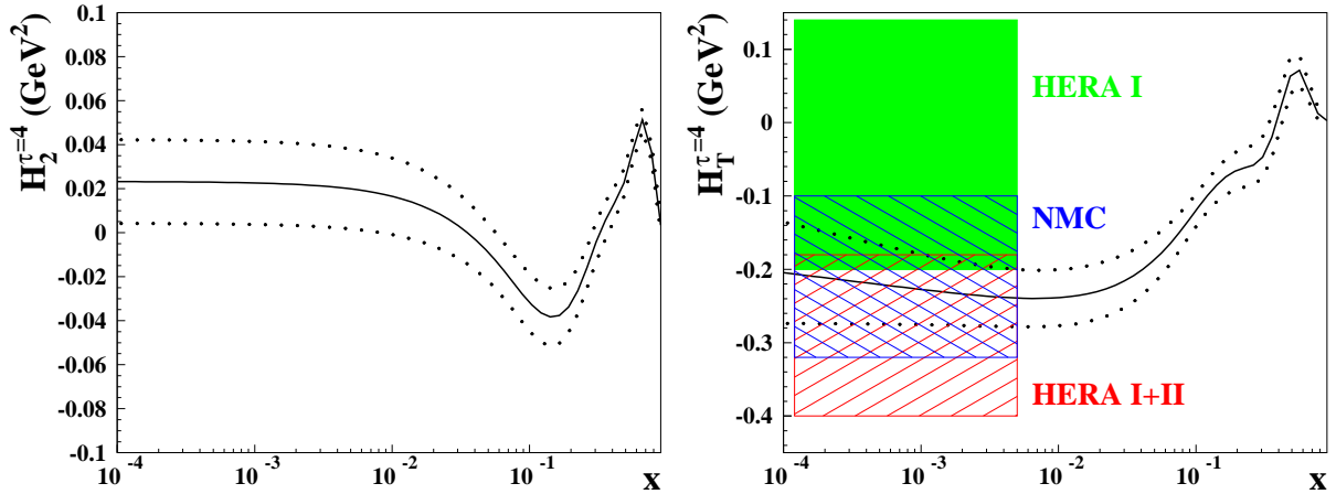
FIG. 26: The coefficients H_2^{\tau=4} (left) and H_T^{\tau=4} (right) in the higher twist terms of the inclusive DIS structure functions, cf. Eq. (6), as a function of x . Shown are the central values (solid) and the 1\sigma bands (dots). The boxes at x \lesssim 5 \cdot 10^{-3} display the low- x asymptotic of H_T^{\tau=4} preferred by the individual data sets indicated (right-tilted hatch: combined HERA run I+II [4], left-tilted hatch: NMC [60], shaded: combined HERA run I [209]).
