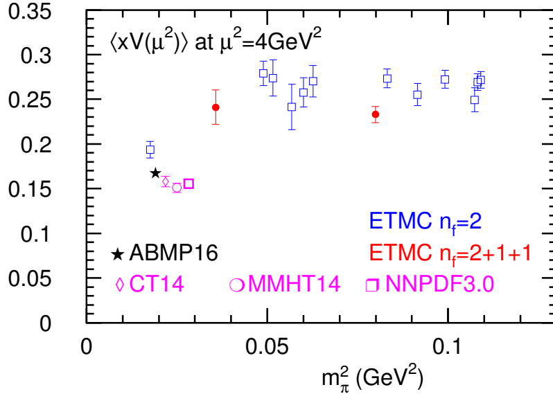
FIG. 32: Lattice computations of Refs. [225–228] for the second moment of the non-singlet distribution xV(\mu^2) at the scale \mu^2 = 4 \text{ GeV}^2 as a function of the pion mass squared, m_\pi^2 , including the uncertainties of the respective measurement compared to the results of ABMP16, CT14, MMHT14 and NNPDF3.0 PDFs given in Tab. IX. The results for CT14, MMHT14 and NNPDF3.0 have been shifted in \Delta m_\pi with respect to ABMP16 for display purposes.
