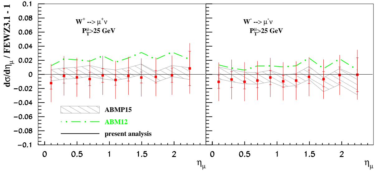
FIG. 8: The same as Fig. 7 for the CMS data on the cross section of inclusive W -boson production at 8 TeV [25].
