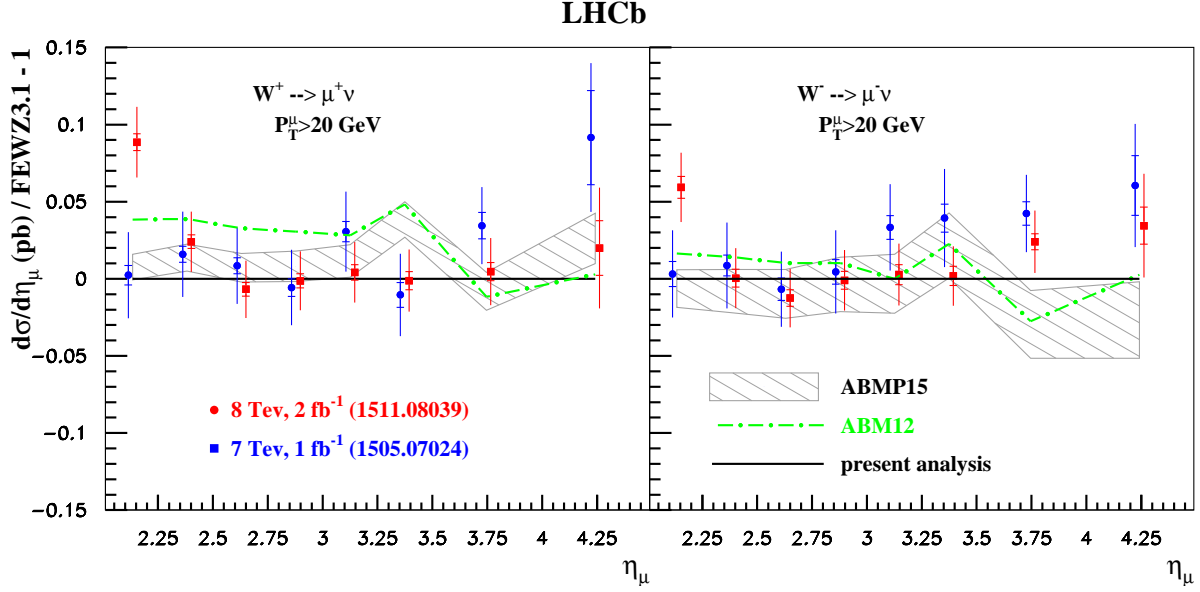
FIG. 10: The same as in Fig. 7 for LHCb data on the cross section of inclusive W -boson production in the pp collision (left: pp \rightarrow W^+ + X \rightarrow \mu^+ \nu + X , right: pp \rightarrow W^- + X \rightarrow \mu^- \nu + X ) at \sqrt{s} = 7 TeV [19] (circles) and \sqrt{s} = 8 TeV [20] (squares) with the muon transverse momentum P_T^\mu > 20 GeV and as a function of the muon pseudo-rapidity \eta_\mu with respect to our fit. The points with the lowest \eta_\mu = 2.125 at \sqrt{s} = 8 TeV are not used in the fit.
