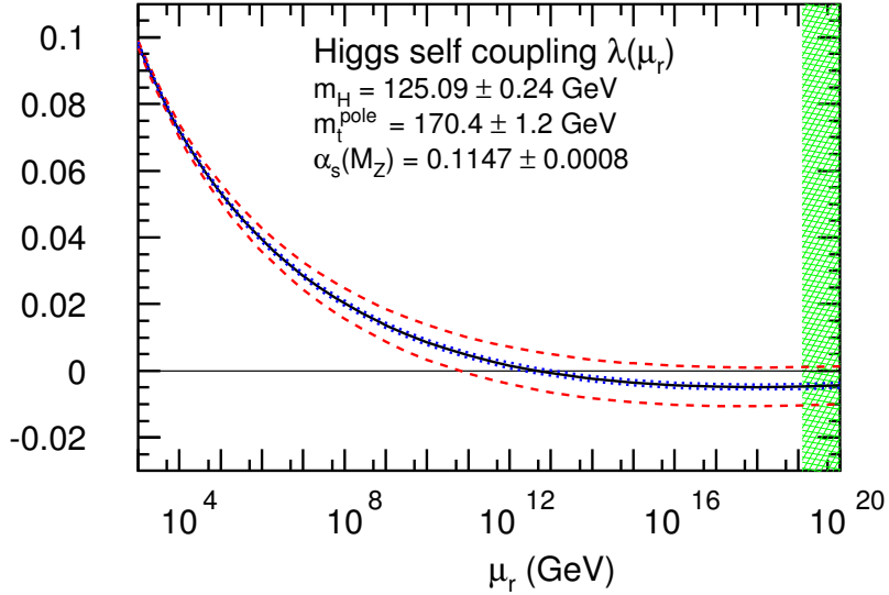
FIG. 34: The renormalization group evolution of the Higgs boson self-coupling \lambda as a function of scale \mu_r . The dashed (red) lines denote the combined 1\sigma uncertainty for \alpha_s^{(n_f=5)}(M_Z) and m_t^{\text{pole}} and the dotted (blue) lines the 1\sigma uncertainty in the value of m_H in Eq. (44). The range of scales \mu_r \geq M_{Pl} is indicated by the hatched (green) band on the right.
