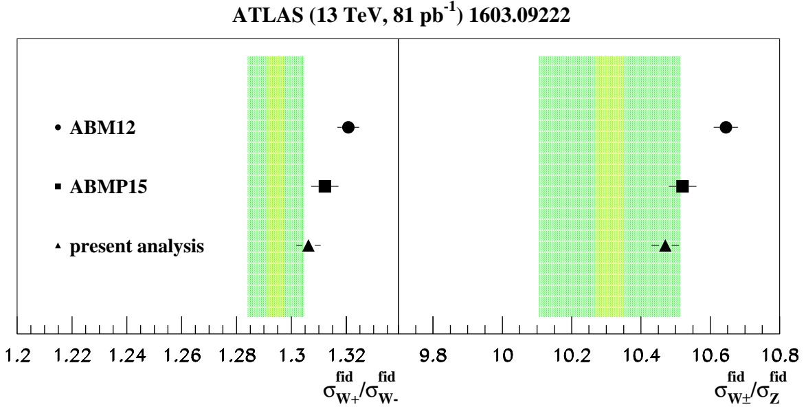
FIG. 13: Cross section ratios for the production of W^\pm - and Z -bosons in the fiducial volume, \sigma_{W^\pm} / \sigma_{W^\pm} (left) and \sigma_{W^\pm} / \sigma_Z (right), in comparison to ATLAS data [26] at \sqrt{s} = 13 TeV together with their 1\sigma PDF uncertainties using the results of our NNLO fit (triangles) as well as ABM12 [1] (circles) and ABMP15 [3] (squares). The inner (yellow) band denotes the statistical uncertainty of the ATLAS data [26] and the outer (green) one the combined uncertainty due to statistics and systematics. The ABM12 predictions are larger than the ones presented in Ref. [26] due to different programs used, FEWZ (version 3.1) [179, 180] and DYNLLO (version 1.5) [200, 201], respectively.
