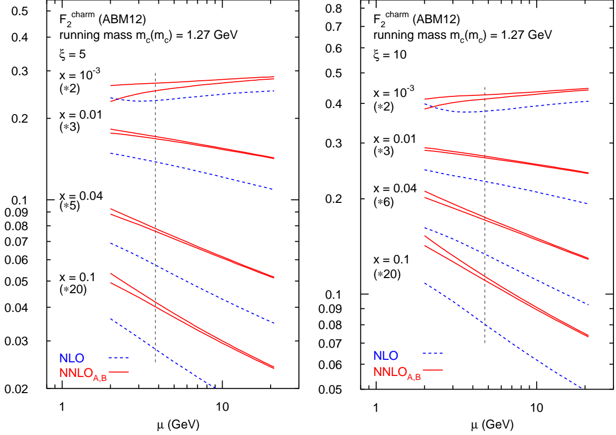
FIG. 3: Scale dependence of the heavy-quark structure function F_2^c for \mu = \mu_R = \mu_F at NLO and at NNLO with the approximations A and B of Eqs. (17) and (18) for two values of \xi = Q^2/m_c^2 . The dashed vertical line denotes the choice \mu = \sqrt{Q^2 + 4m_c^2} .
