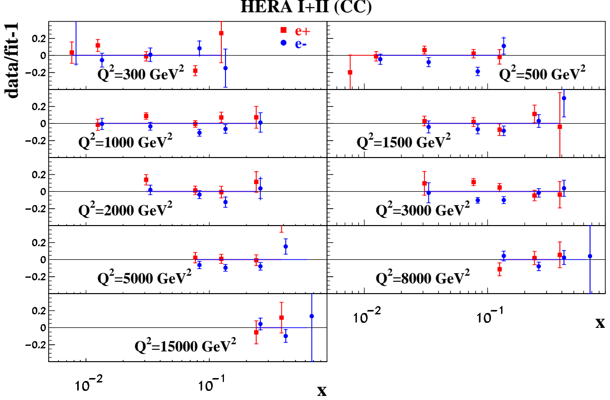
FIG. 6: The same as in Fig. 4 for the CC e^+p (squares) and e^-p (circles) inclusive DIS data [4] versus Bjorken x in bins of the momentum transfer Q^2 .
