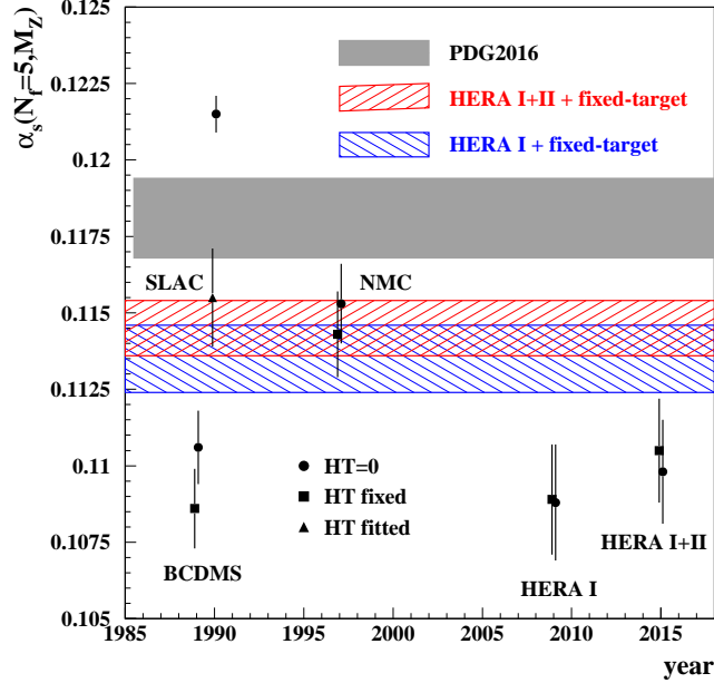
FIG. 29: The value of \alpha_s^{(n_f=5)}(M_Z) in the \overline{\text{MS}} scheme for n_f = 5 at NNLO in QCD determined by the individual data sets as a function of the year of their publication. Data from SLAC [54, 56, 62] (proton), BCDMS [61], NMC [60] (proton), the HERA run I [209] as well as the HERA run I+II combination [4] are considered in three variants for the treatment of the higher twist terms defined in Eq. (6): (i) the higher twist terms are set to zero (circles); (ii) the higher twist terms are fixed to the values obtained in the ABMP16 fit from considering all data sets (squares); (iii) the higher twist terms are fitted to the individual data set under study (triangles). The bands for \alpha_s^{(n_f=5)}(M_Z) obtained by using the combination of the SLAC, BCDMS and NMC samples together with those from the HERA run I (left-tilted hatches) and the run I+II combination (right-tilted hatches) as well as the 2016 PDG average [212] (shaded area) are presented for comparison.
