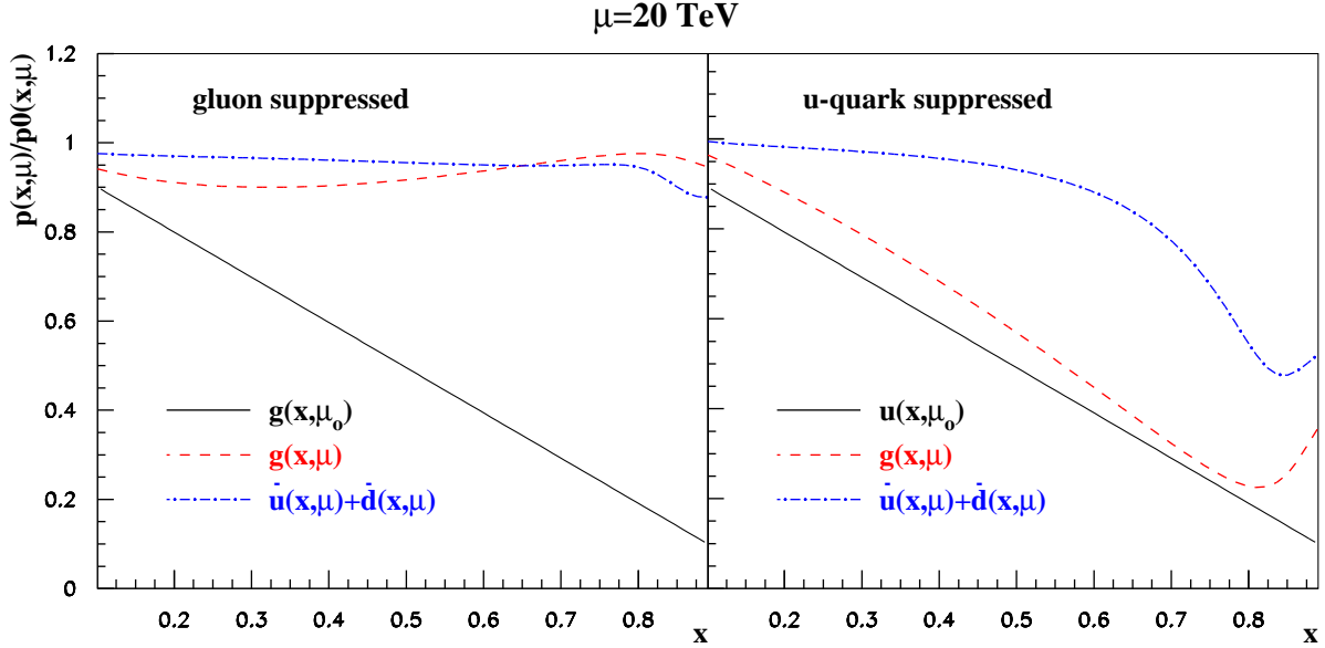
FIG. 21: A response of the gluon (dashes) and non-strange sea (dashed dots) distributions evolved from the factorization scale \mu_0 = 3 GeV to \mu = 20 TeV to the suppression of the initial gluon distribution g(x, \mu_0) (left panel) and up-quark distribution u(x, \mu_0) (right panel) by a factor of (1 - x) (solid lines) given as a ratio of PDFs p(x, \mu) and p_0(x, \mu) with and without suppression, respectively.
