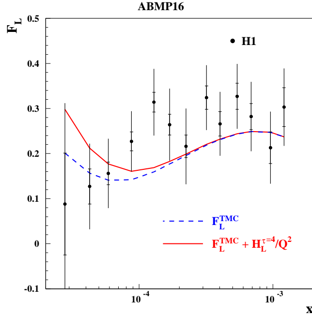
FIG. 27: The data on the longitudinal structure functions F_L as a function of x by the H1 collaboration at HERA [210] compared to the predictions of our analysis at NNLO in QCD based on either including higher twist terms (solid) or setting them to zero (dashes), cf. Eq. (6).
