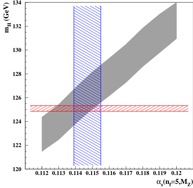
FIG. 33: The value of Higgs-boson mass m_H computed according to the condition in Eq. (45) for vacuum stability at M_{Pl} using the values of m_t with their uncertainties obtained in the present analysis by scanning \alpha_s^{(n_f=5)}(M_Z) in the range of 0.112 \div 0.120 and disregarding the theoretical uncertainty of \pm 0.3 GeV (gray band). For comparison the 1\sigma bands for \alpha_s^{(n_f=5)}(M_Z) from the nominal fit and the value of m_H in Eq. (44) (left-tilted and right-tilted hatch, respectively) are shown.
